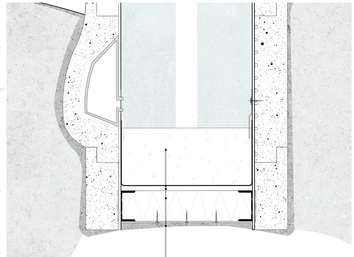
Detail B 1:10
