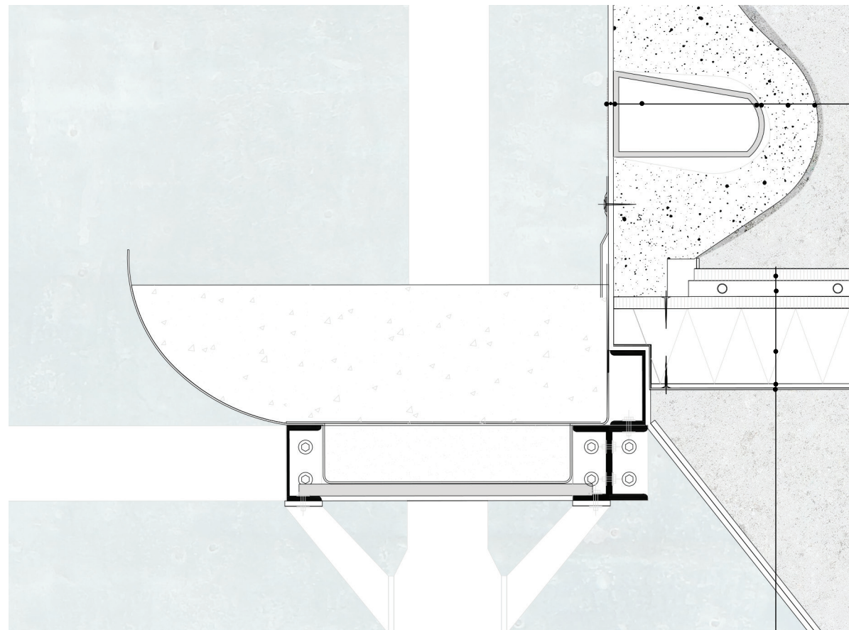
Detail C 1:10
