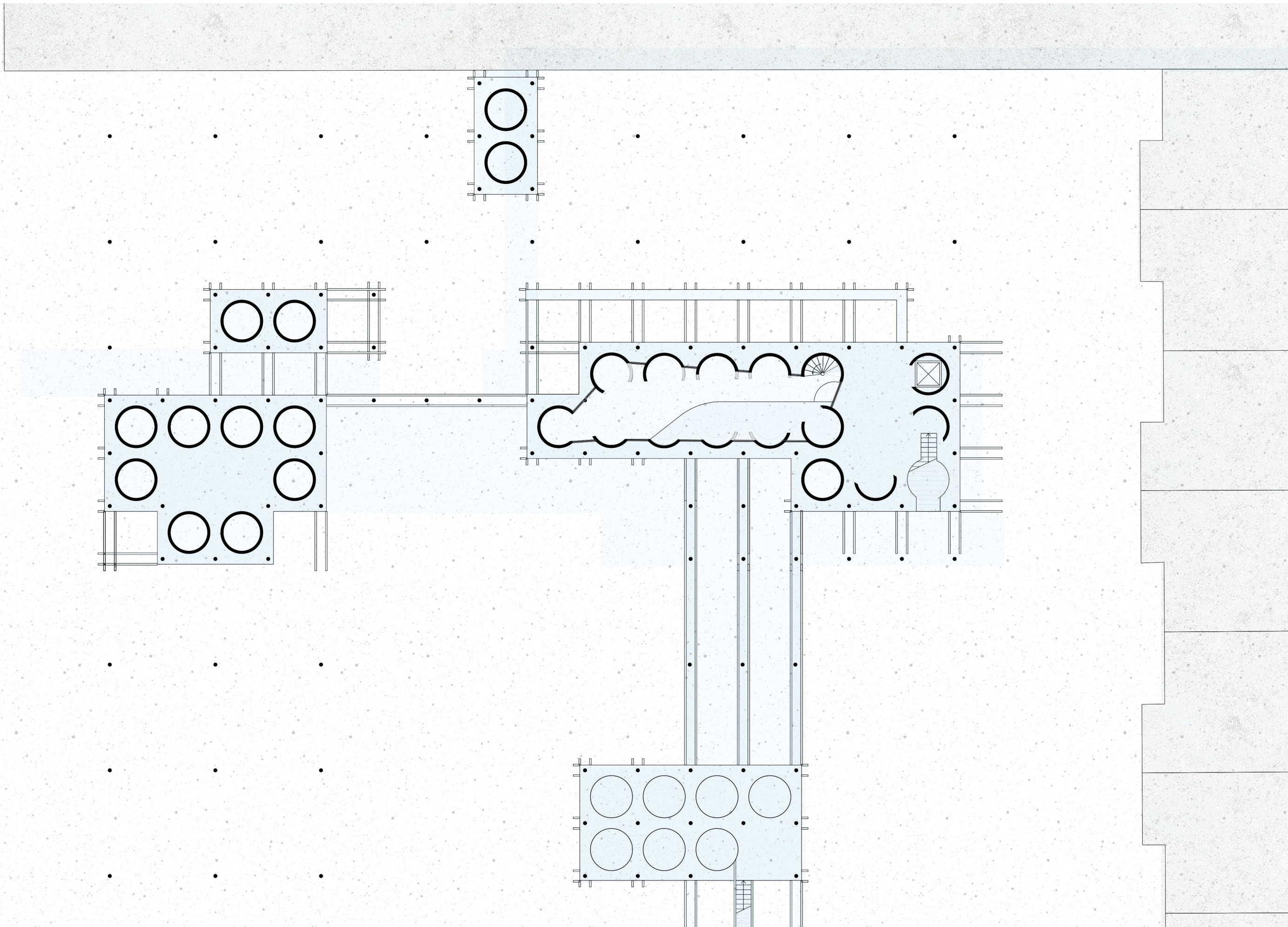
second floor 1:200
