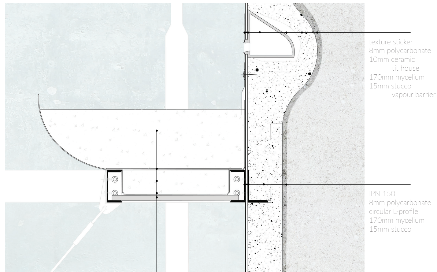
Detail A 1:10
