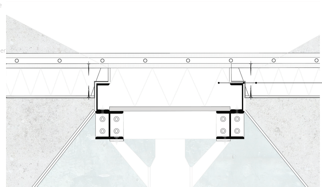
Detail D 1:10
