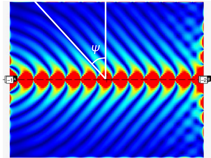
Fig. 12 Snapshot of the current distribution J_{xy} around a straight CPW. \Psi = \arccos(\sqrt{\epsilon_{\text{eff}}/\epsilon_r}) = 42.5^\circ is derived from \epsilon_{\text{eff}} = 6.22 of the CPW line calculated by Sonnet and \epsilon_r = 11.44 of the Si substrate. Note that the current densities plotted do not represent de-embedded data, and therefore areas near any port include the effect of the port discontinuity, according to the manual of Sonnet (Video 2, .mov, 6.71 MB [URL: https://doi.org/10.1117/1.JATIS.8.3.036005.s2 ]). 16
