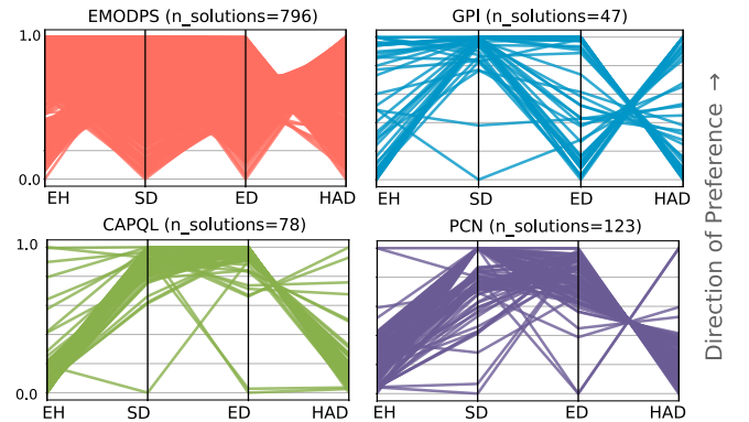
Figure 6: Parallel coordinate plots for the Nile WMS.
