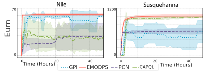
Figure 5: Expected Utility over time
