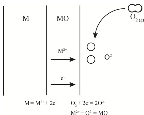
Figure 2.1: A schematic of the processes that contribute to the growth of an oxide scale through reactions and transport.
