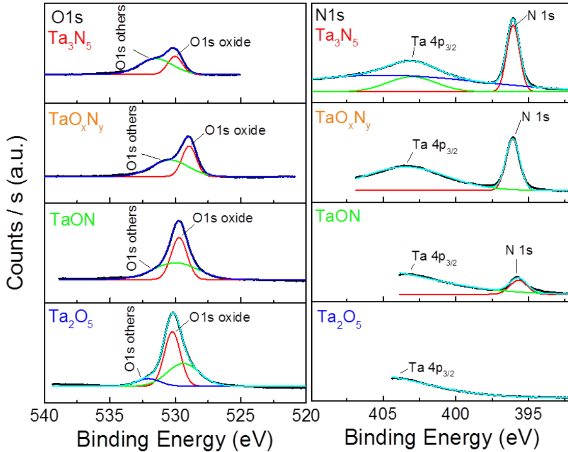
Figure 4.9. XPS surface data showing the O-1s and N-1s signals of (from bottom to top): Ta film oxidized in air at 650°C, Ta_2O_5 in blue; Ta film annealed at 827°C at p_{NH_3}/p_{H_2}=0.01 and p_{NH_3}/p_{H_2} = 0.1 , \beta -TaON in green; Ta film at 0.3 \leq p_{NH_3}/p_{H_2} \leq 3 , mixed TaON and Ta_3N_5 in orange; the top-most pattern belongs to a Ta film annealed at p_{NH_3}/p_{H_2} = 10 , Ta_3N_5 in red. Sample charging was observed for the Ta_2O_5 , \beta -TaON and for the mixed phase TaON- Ta_3N_5 samples, while no charging was observed in the Ta_3N_5 film. The C1s peak (285.2 eV) was used as a standard to calibrate the binding energies.
