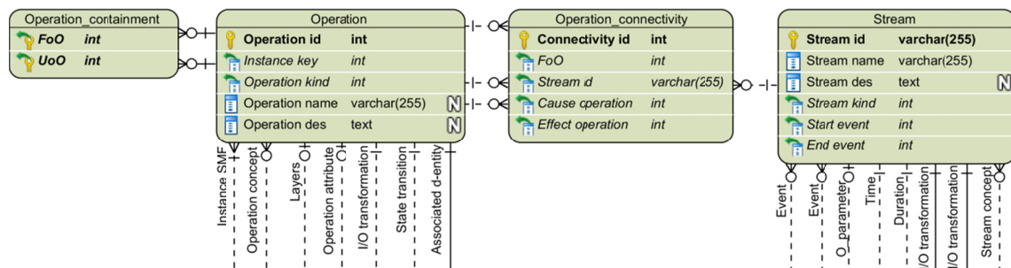
Figure 5-46 Construct for capturing operation containment and connectivity relationships of SMF instances
