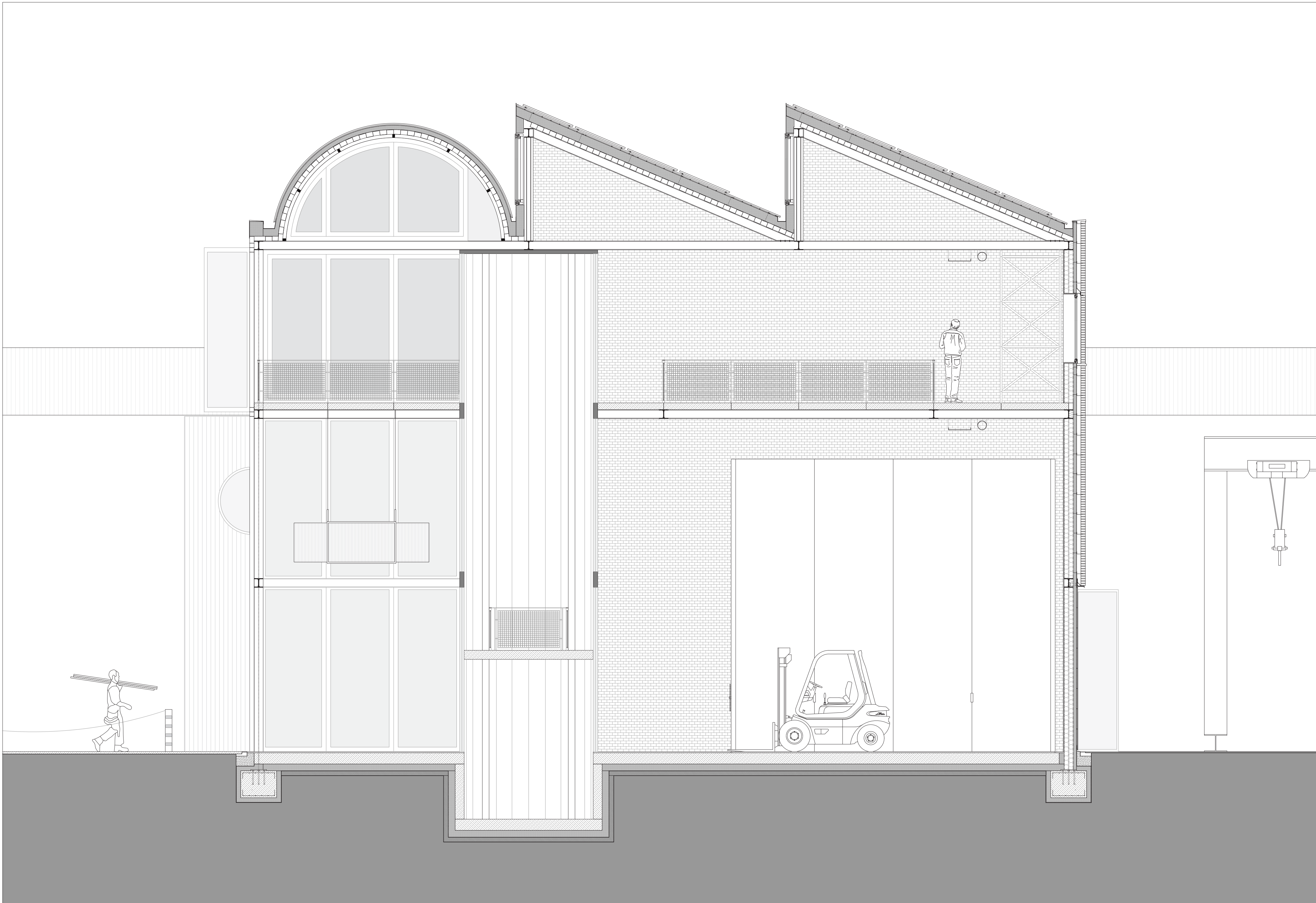
1:50 section
