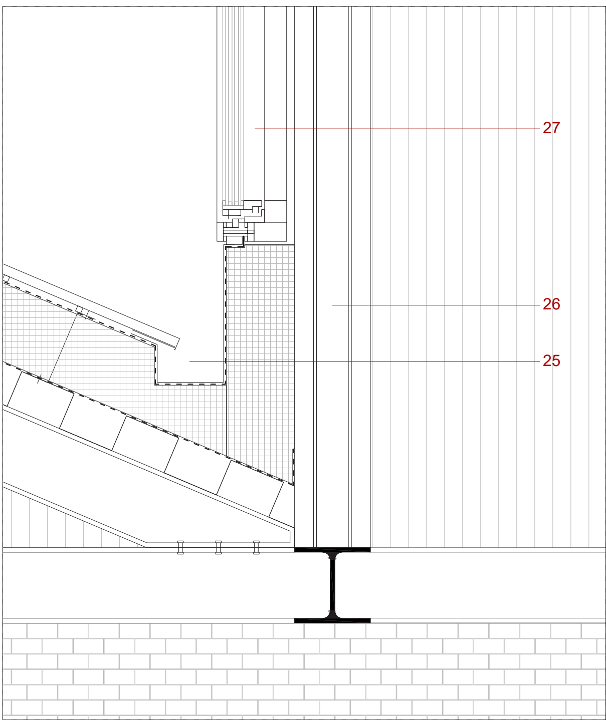
1:5 roof details
