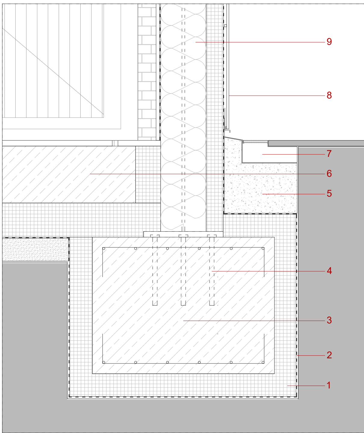
1:5 facade details
