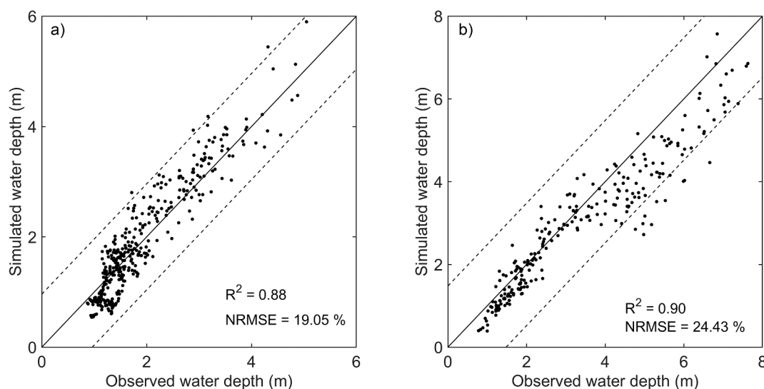
Fig. 5. Results of model calibration and validation for Cross-Section A (Fig. 3). a) Model calibration: observed vs simulated maximum water depth - September 1972 to September 1973 (maximum discharge 1,362 \text{ m}^3/\text{s} ). b) Model validation: observed vs simulated maximum water depth - January 1980 to February 1981 (maximum discharge 1,868 \text{ m}^3/\text{s} ). 1:1 relationship in solid line; dashed lines represent the range of the deviation by 1.5 times the average measured water depth in the respective periods of calibration and validation. The NRMSE is calculated as the RMSE normalized by the average measured water depth.
