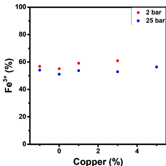
Fig. 8. \text{Fe}^{3+} content obtained from fitting Fe 3p region. The reference \text{Fe}_3\text{O}_4 value is shown at -1% on the x-axis. The fits are provided in the supporting info (Fig. S1).
