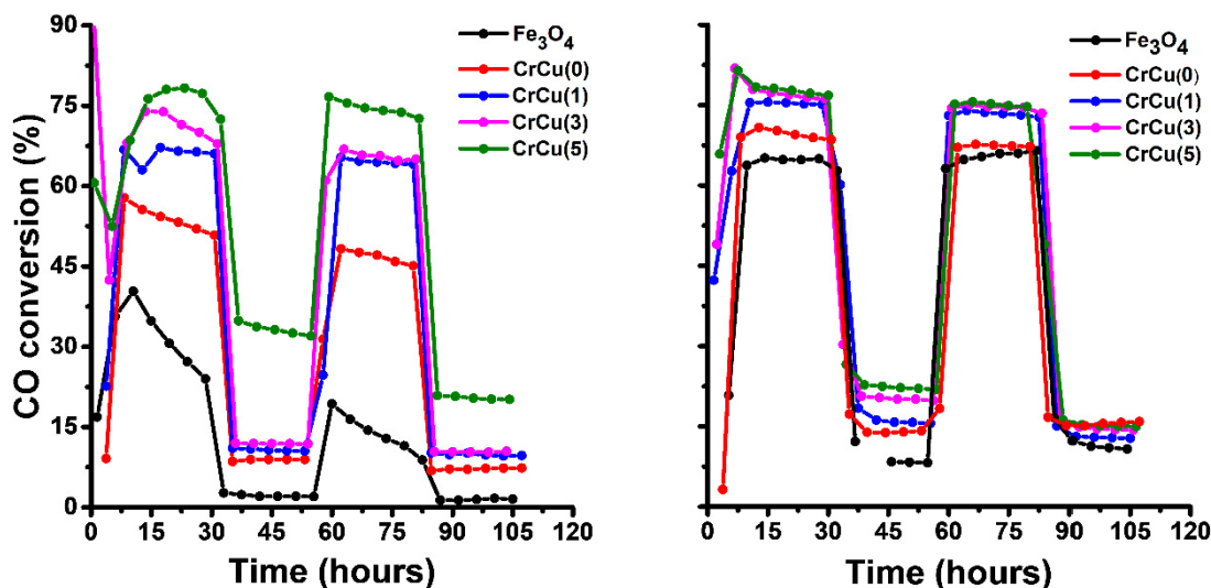
Fig. 3. CO conversion over time at 2 bar (left) and 25 bar (right). The \alpha - \text{Fe}_2\text{O}_3 phase present in the \alpha - \text{Fe}_2\text{O}_3 (ref) catalyst is transformed into \text{Fe}_3\text{O}_4 during the reaction. CO conversion of the \text{Fe}_3\text{O}_4 and CrCu(0) reference catalysts at 25 bar were recorded in a separate run than the samples characterised in the next section.
