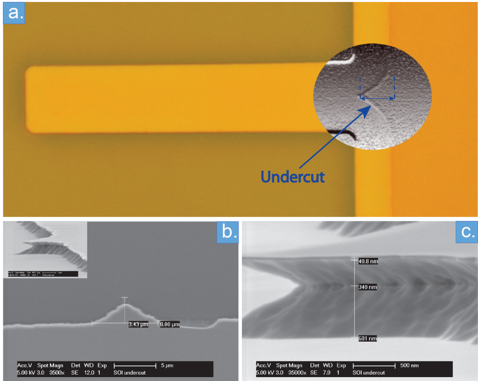
Figure 6. (a) Optical microscope image of a cantilever with hidden anchor due to under etching of the base of the cantilever. (b) SEM of a hidden anchor. The cantilever was forcibly removed in order to see the hidden anchor. The inset shows the bonding surfaces of the SOI wafers were in the middle of the BOX layer. (c) Close-up view of bonding interface and silicon device layer.
