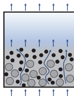
Figure 11.5 Graphical presentation of anaerobic plug-flow feeding through a bed of settled granules in an aerobic sludge reactor.
