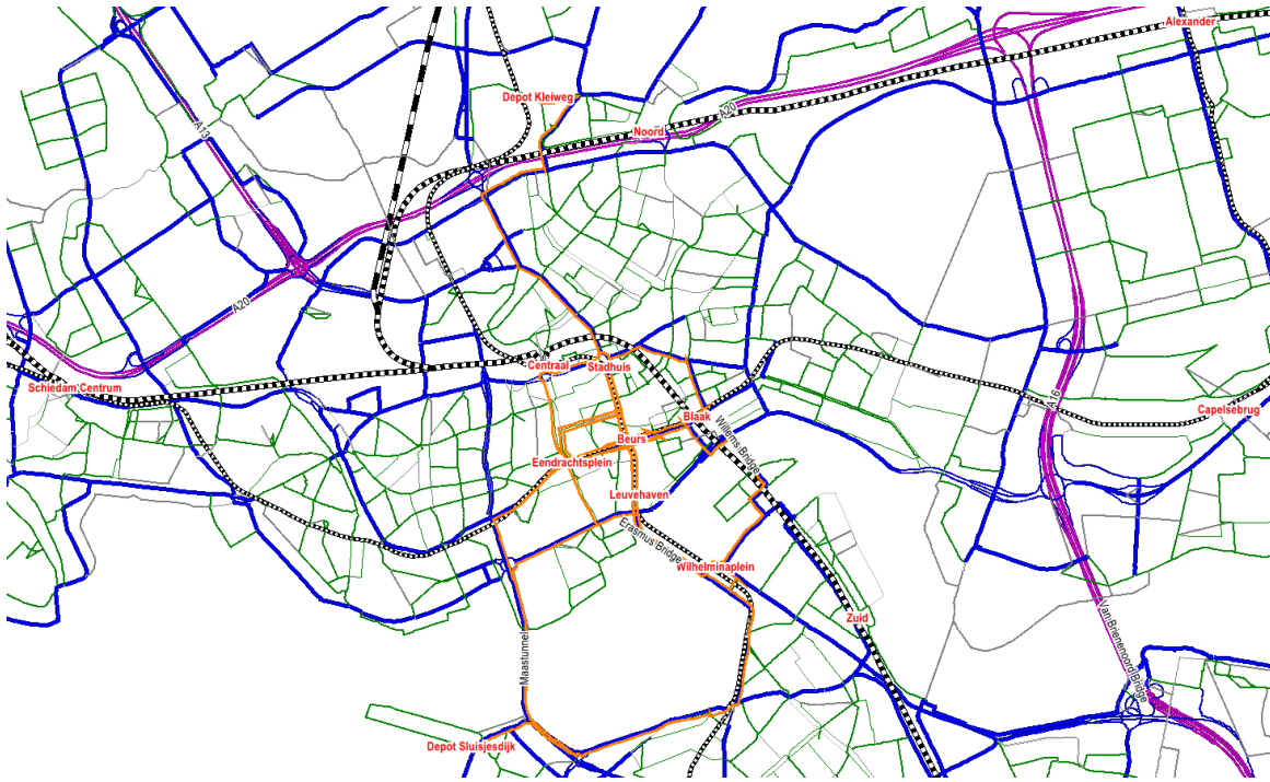
FIGURE 4 Excerpt of the simulated multimodal network with the road links for bus bridging highlighted (orange).
