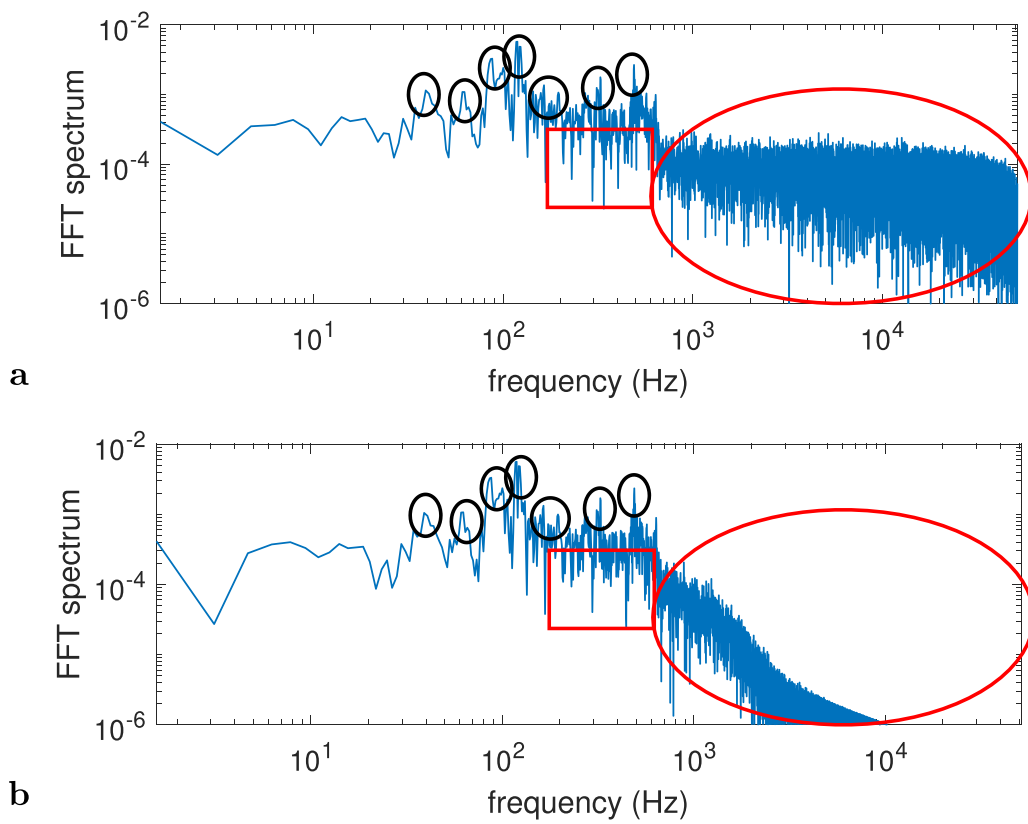
Figure 20. The FFT spectra of (a) the original signal and (b) the despeckled signal.
