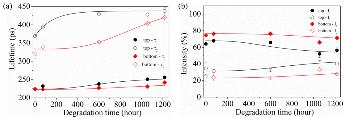
FIG. 9. (a) Positron lifetime \tau_1 and \tau_2 , and (b) intensity I_1 and I_2 for the top and bottom layer of the ZnO:Al TCO of a CIGS solar cell as a function of time of accelerated degradation. Full lines are guides to the eye.
