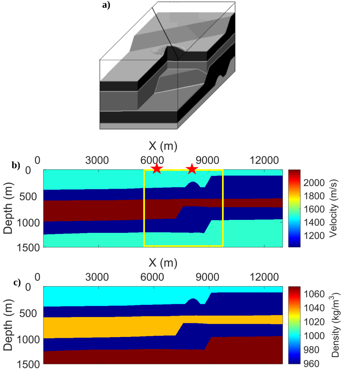
Figure 6.1: (a) The 3D physical model, (b) the velocity model of the scaled 2D cross section along the acquisition line, red stars indicate source positions of two reflection responses shown in Figure 6.2, the yellow box marks the target zone which is imaged, (c) the density model of the scaled 2D cross section along the acquisition line.
