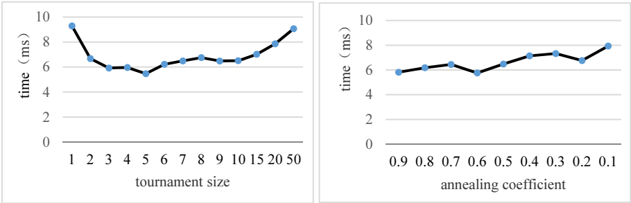
Figure 3. Effects of tournament sizes and annealing coefficients.
