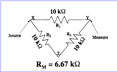
Figure 4. A measured value between X and Y of 6.67 k \Omega is correct, while R_1 is a 10 k \Omega device [7].
