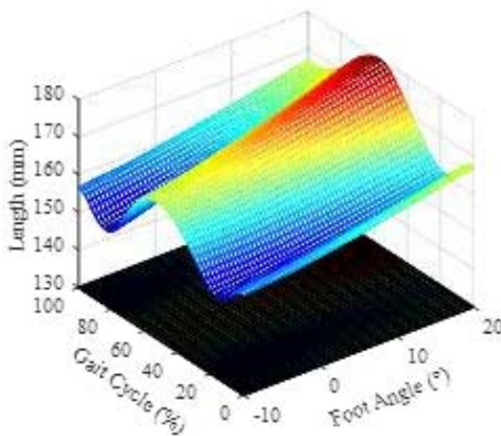
Figure 8. The effect of the foot angle around the sagittal axis on Adductor Longus.
