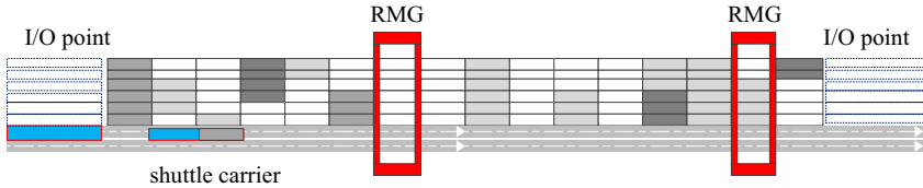
Figure 3. New configuration of container storage yard.
