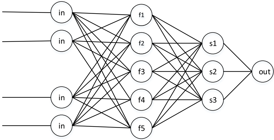
Figure 1. Structure of improved GPN algorithm.
