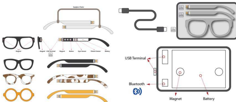
Figure 4. Main Products Architecture & Case Products Architecture.
