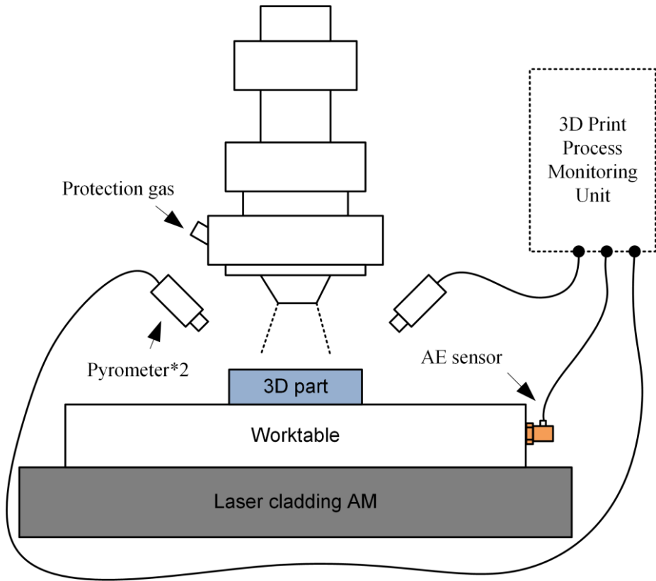
Figure 2. Experimental setup.
