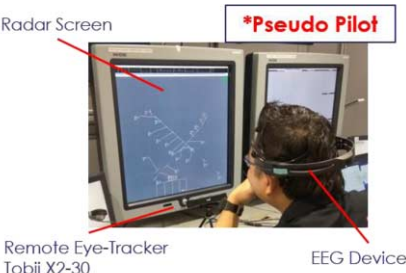
Figure 2. Controller Working Position with equipment required
