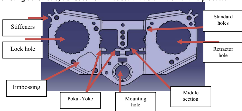
Figure 1. Structural design of the seat belt retractor housing.
