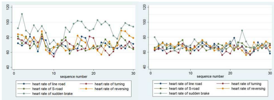
Figure 2. HR of sudden brake and mean HRs of four driving situations on scooter (left) and motor wheelchair (right).
