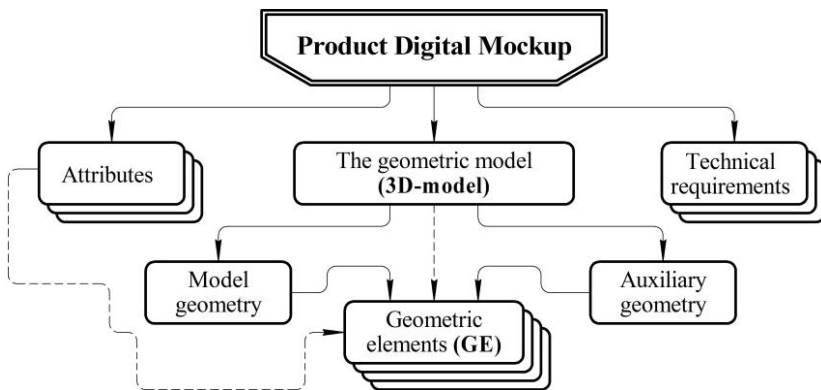
Figure 1. Product digital mockup structure
