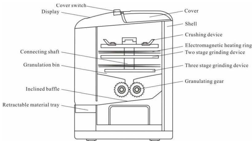
Figure 4. Structure diagram of organic waste processor.
