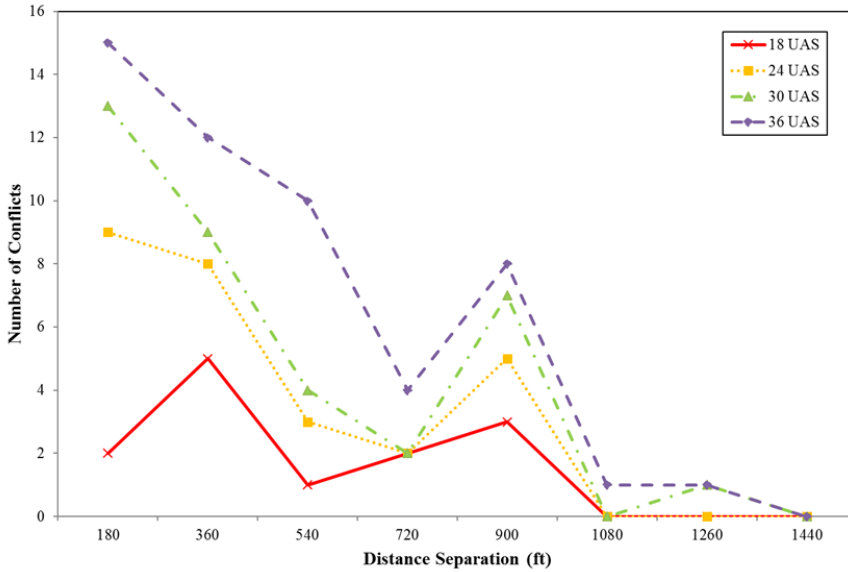
Figure 3. Number of conflicts with respect to distance separation with speed control algorithm.
