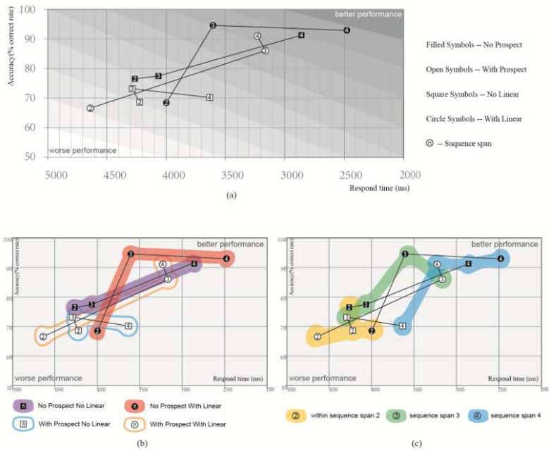
Figure 4. Comparison illustration of the mean performance in the same trial (4-a) show the overall distribution of means performance among the trials; (4-b) the bubbles represent four different displayed experimental material conditions; (4-c) the bubbles represent three kinds of temporal order span
