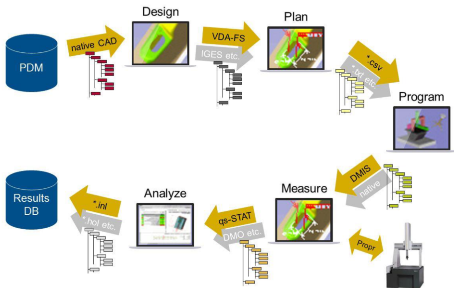
Figure 1. Interfaces in a typical measuring process.
