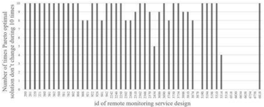
Figure 5. Number of times Pareto optimal solution remained as randomly increasing characteristic values.
