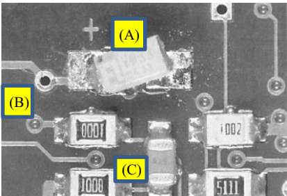
Figure 6. (A) An off-registration or off-pad component, (B) VIA holes linked to SMT pad/components allowing ICT test system to assess the SMT components for measurements and (C) notices that 2 SMT component pads is linked together without any visible VIA holes for use as test node [7].
