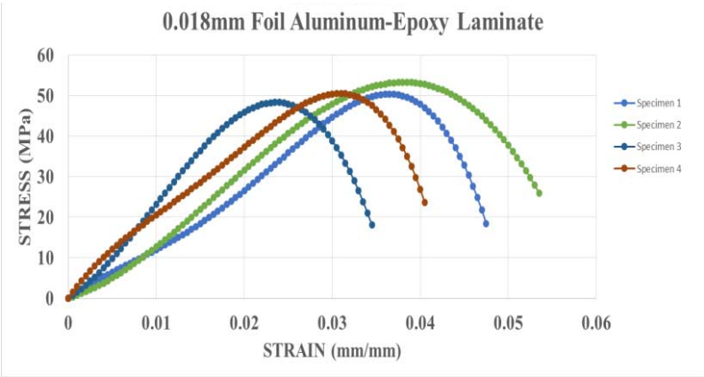
Figure 9. Stress-Strain diagram of foil Aluminum-Epoxy Laminate.
