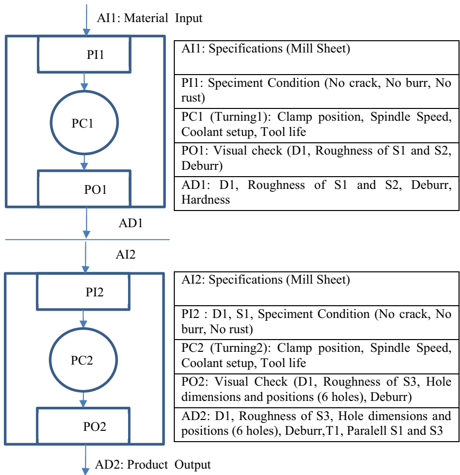
Figure 3. MAP chart for Hub-flange manufacturing process in company X.
