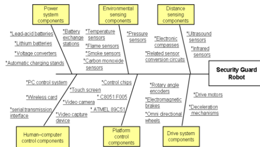
Figure 2. Key Components of the Security guard robot.
