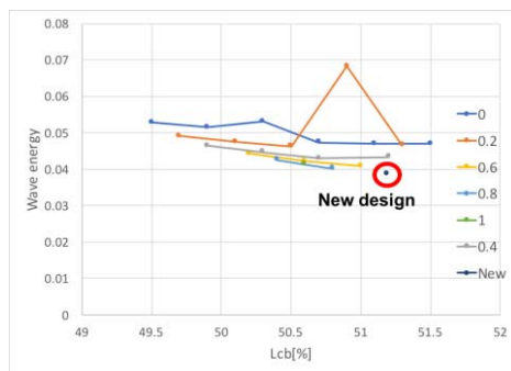
Figure 6. Results of Rankine source method (with process data).
