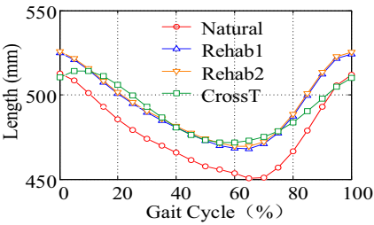
(e1) Comparison of Semitendinosus length
