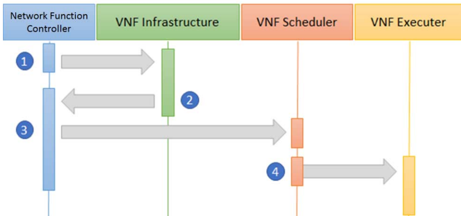
Figure 4. Time Sequence of Network Function Controller Component.
