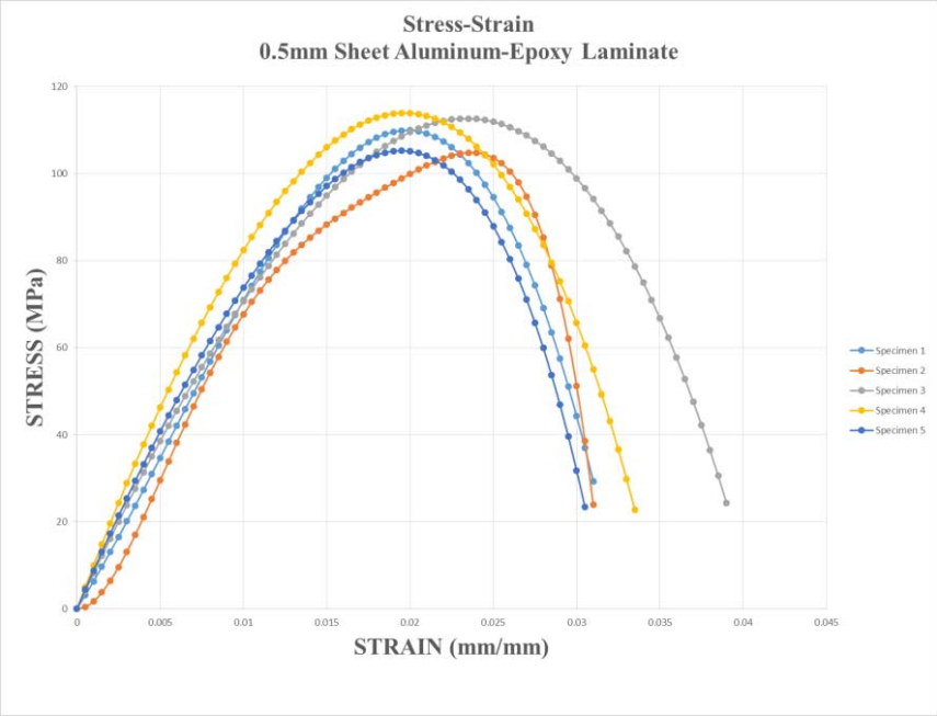
Figure 8. Stress-Strain diagram of sheet Aluminum-Epoxy Laminate.
