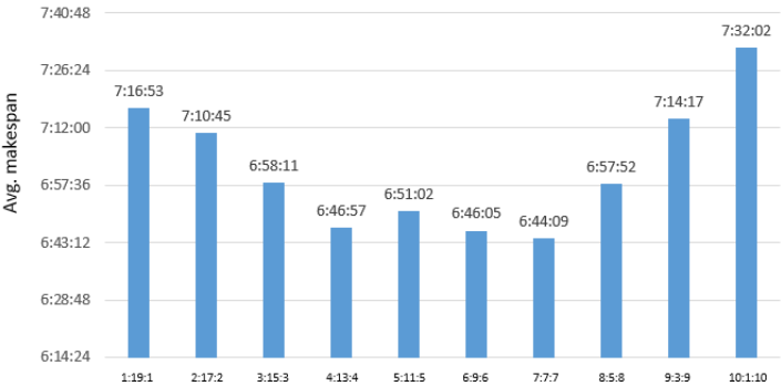
Figure 12. Performance with different yard block division.
