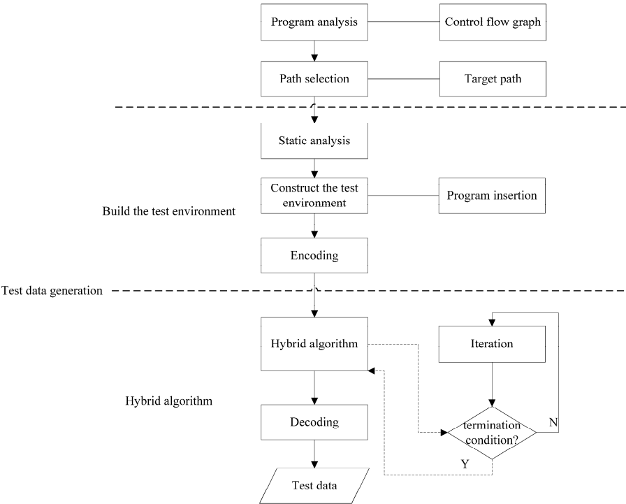
Figure 1. Test data generation process.
