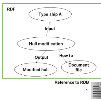
Figure 3. Example of process data on RDF.
