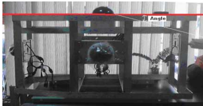
Figure 6. Test Stand and Camera 1.
