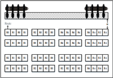
Figure 2. Yard template of cost-saving pattern..
