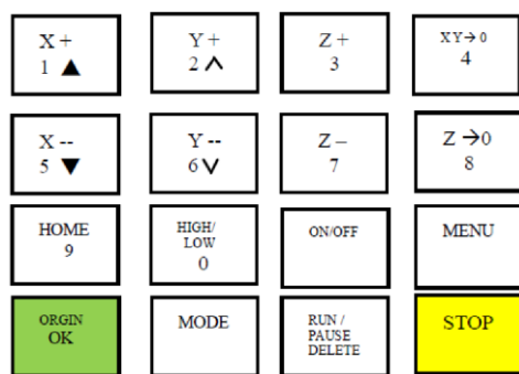
Figure 2. Keyboard placement of handheld manipulator.
