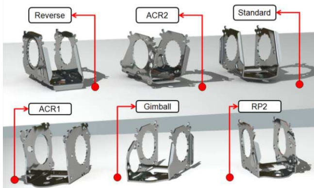
Figure 6. Alternative retractors housings as result models from Generative Model.
