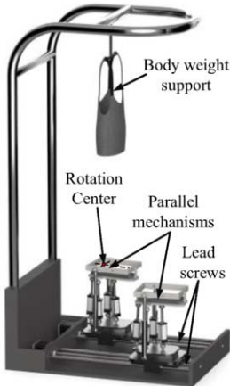
Figure 4. CAD model of the rehabilitation robot.
