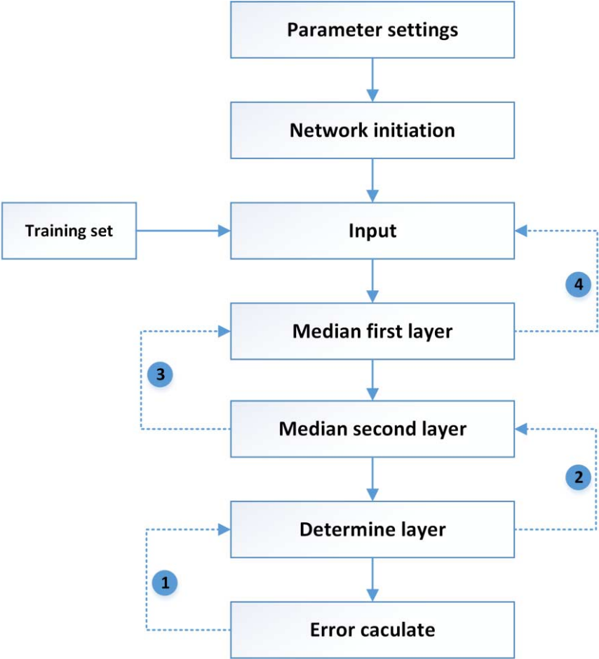
Figure 2. Procedure of improved GPN algorithm.
