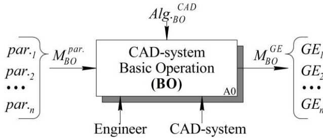
Figure 3. CAD-system basic operation process diagram in IDEF0 notation
