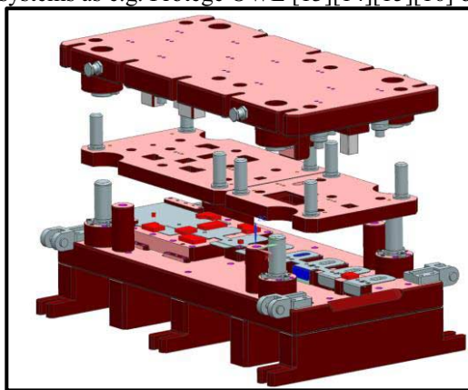
Figure 1. Multi-stage stamping die.
