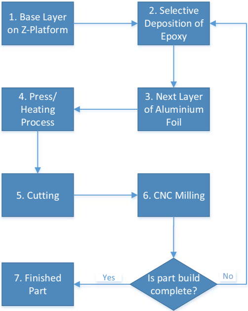
Figure 7. Flow diagram of laminate printing process
