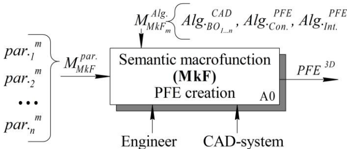
Figure 6. Semantic macrofunction process diagram in IDEF0 notation
