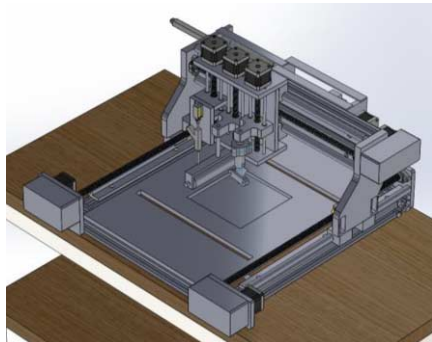
Figure 3. Isometric CAD Model.
