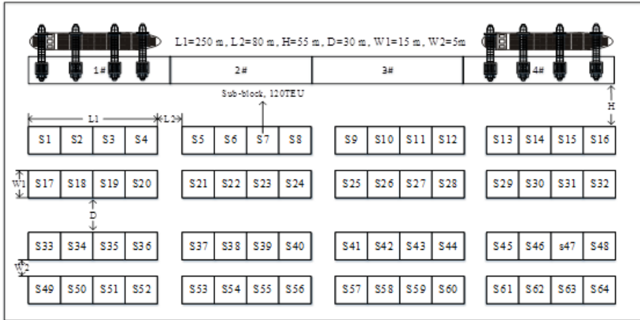
Figure 1. Terminal yard configuration
