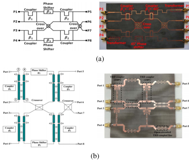
FIGURE 31. Flexible phase difference 4x4 Butler matrices: (a) [103], (b) [104].
