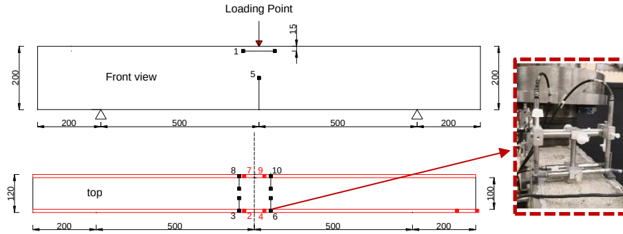
(b) LVDT arrangement for strengthened beam (Unit: mm)
