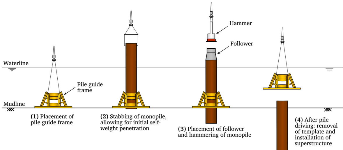
Fig. 1. Example of a monopile installation process.
