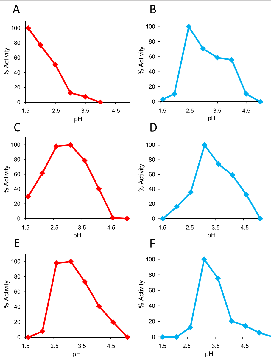
Figure 5 Optimal pH for VA (left) and RB5 (right) oxidation by S168W (A and B) and S168W-environment (C and D) variants of C. subvermispura MnP6, and native P. ostreatus VP1 (E and F). Activities for 6 mM VA (A, C, and E) and 15 \mu M RB5 (B, D, and F) oxidation by the S168W (A and B) and S168W-environment (C and D) variants, and native VP1 (E and F) were estimated in 100 mM BR buffer of pH 1.6 to 5.0. Means from triplicate experiments.
