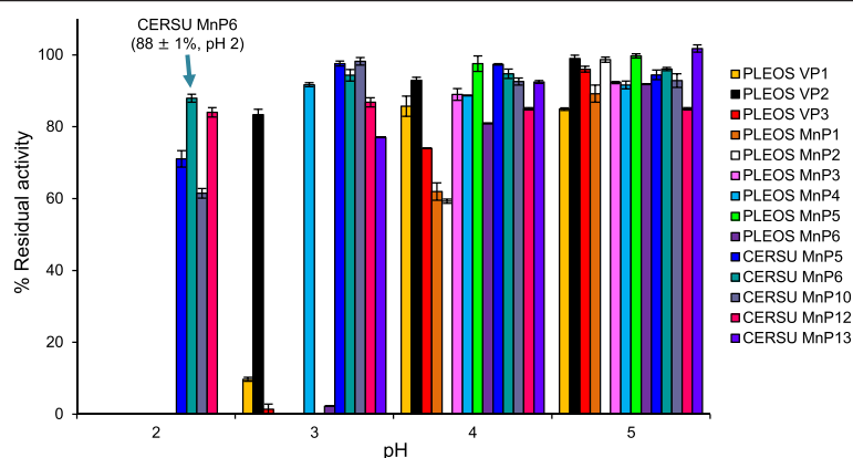
Figure 1 Acidic pH stabilities of 14 ligninolytic peroxidases from the P. ostreatus and C. subvermisporea genomes. Residual activities of P. ostreatus (PLEOS) VP1 (PC9 genome model 137757), VP2 (PC15 genome model 1113241), VP3 (PC15 genome model 156336), short MnP1 (PC15 genome model 1096331), short MnP2 (PC15 genome model 199510), short MnP3 (PC15 genome model 1089546), short MnP4 (PC15 genome model 1099081), short MnP5 (PC15 genome model 199511), and short MnP6 (PC15 genome model 1041740) and C. subvermisporea (CERSU) extralong MnP5 (genome model 49683), extralong MnP6 (genome model 50686), long MnP10 (genome model 117436), long MnP12 (genome model 157986), and short MnP13 (genome model 124076), after 24-h incubation at 4°C, in 100 mM Britton-Robinson (BR) buffer of pH 2.0 to 5.0. Means and 95% confidence limits from triplicate experiments.
