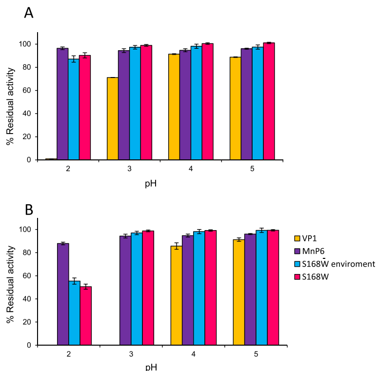
Figure 4 pH stabilities of the S168W and S168W-environment variants of C. subvermispota MnP6 compared to the native MnP6 and the P. ostreatus VP1 after 4-h (A) and 24-h incubation (B). Residual activities were determined by 1.5 mM Mn 2+ oxidation in 0.1 M tartrate, pH 5.0, after incubation at 4°C, in 100 mM BR buffer, pH 2.0 to 5.0. Means and 95% confidence limits from triplicate experiments.
