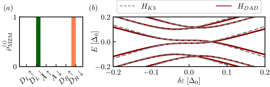
Figure 3.4: (a) Majorana wavefunctions at the sweet spot of a dot-ABS-dot chain. (b) Energy spectrum of the system as a function of detuning energy \delta\varepsilon . The solid lines are calculated for the full many-body Hamiltonian, while the grey dashed lines are based on the low-energy effective theory. The energy splitting at \delta\varepsilon = 0 is due to effective next-nearest-neighbor coupling between the two outer dots.
