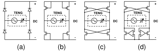
Fig. 7. Different configurations of full-bridge rectifiers in triboelectric energy harvesting. (a) Passive diode rectifier; (b) Diode-connected gated rectifier; (c) Cross-coupled rectifier; (d) Active-diode rectifier [46].
