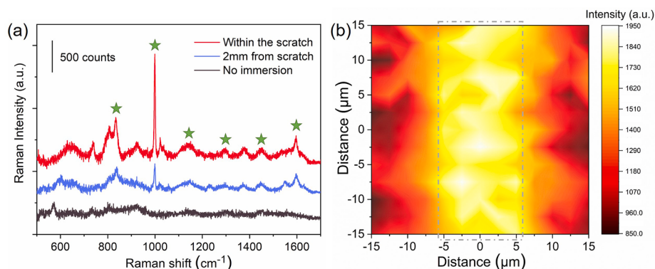
Fig. 7. (a) Raman spectra of BTA molecules on AA2024-T3 substrate surface at different detection positions; (b) Raman intensity mapping of BTA at 1010\text{ cm}^{-1} over an area of 30 \times 30\text{ }\mu\text{m}^2 within the scratch, and X axial direction was perpendicular to the scratch line.
