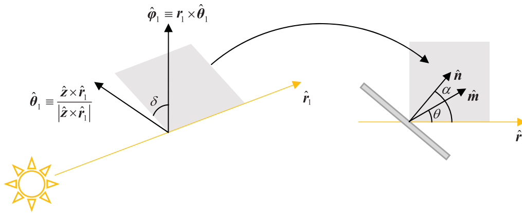
Fig. 4 Solar-sail pitch and clock angles defined with respect to frame S(\hat{r}_1, \hat{\theta}_1, \hat{\varphi}_1) . Adapted from Ref. [26].
