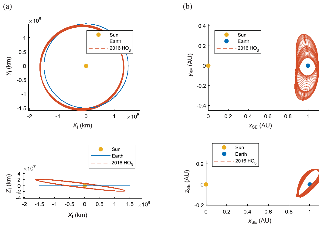
Fig. 1 Orbit of 2016 HO 3 in the 1960–2020 timeframe: (a) in the inertial frame A(X_1, Y_1, Z_1) ; (b) in the synodic Sun–Earth frame B_{SE}(x_{SE}, y_{SE}, z_{SE}) .
