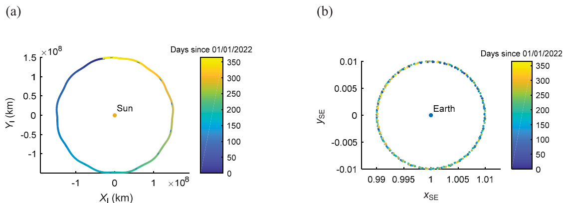
Fig. 6 Conditions at the Earth's sphere of influence of the trajectory in Fig. 5 for the year 2022: (a) in the inertial frame A(X_I, Y_I, Z_I) ; (b) in the synodic Sun–Earth frame B_{SE}(x_{SE}, y_{SE}, z_{SE}) .
