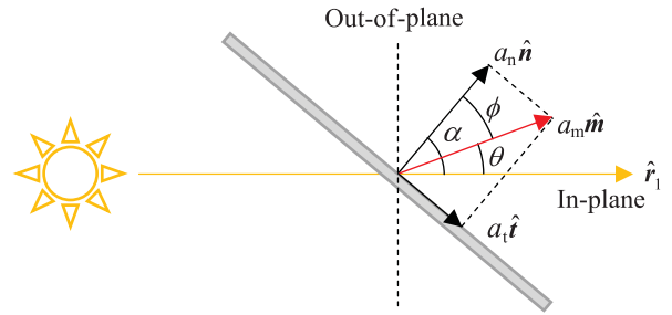
Fig. 3 Side-view schematic of non-ideal solar-sail acceleration components.
