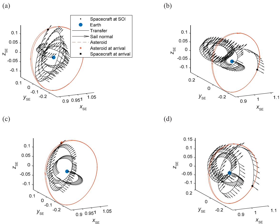
Fig. 7 Solar-sail case—best initial guess trajectories in the synodic Sun–Earth frame B_{SE}(x_{SE}, y_{SE}, z_{SE}) for an ideal solar-sail model and for (a) \beta = 0.025 , (b) \beta = 0.03 , (c) \beta = 0.035 , and (d) \beta = 0.04 .
