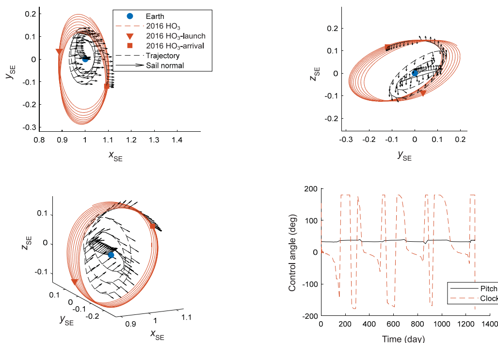
Fig. 9 Solar-sail case—optimized trajectory and controls for ideal sail model and \beta = 0.025 .
