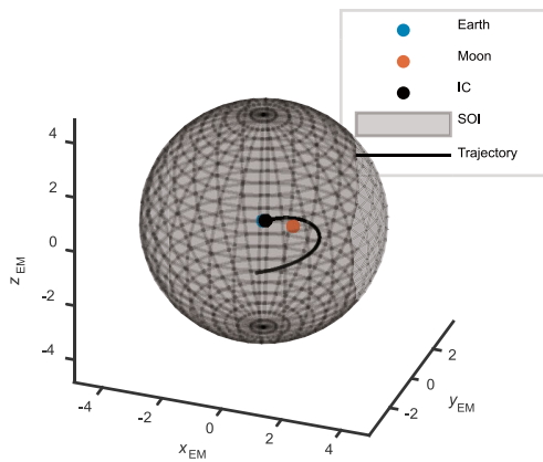
Fig. 5 Ballistic trajectory starting from the initial condition in Eq. (1) depicted in the synodic Earth–Moon frame B_{EM}(x_{EM}, y_{EM}, z_{EM}) .
