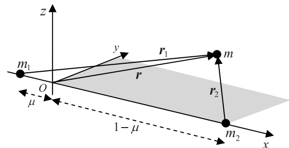
Fig. 2 Schematic of circular restricted three-body problem.
