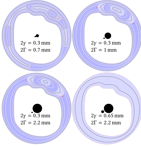
Fig. 14. Variable-width contouring on Jin's ring [Jin et al. 2017a] with various values of \gamma and \Gamma . Underfill in red. There is no overflow.
