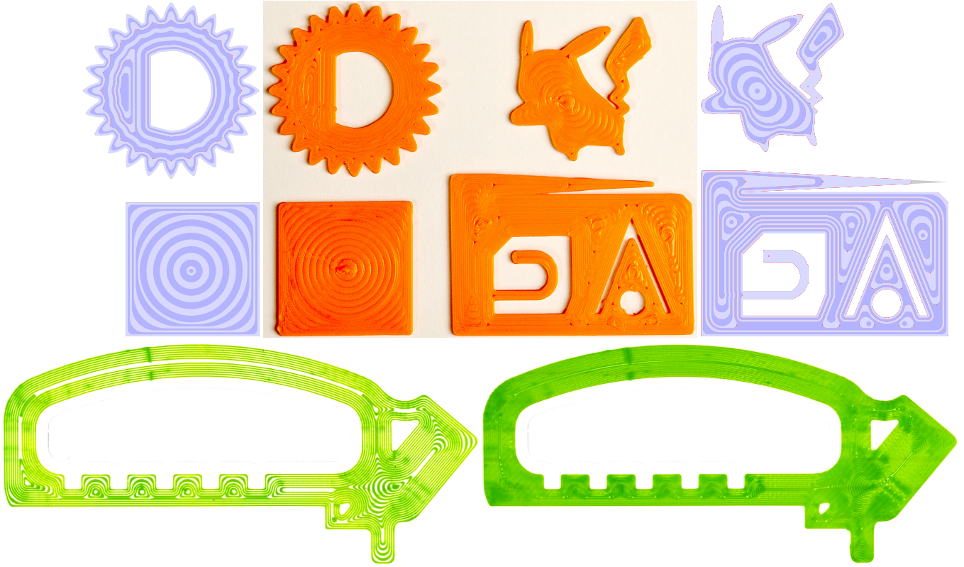
Fig. 18. Top . Photographs of prints obtained on an Ultimaker 2+ system (processed to bring out details). Each sample is 4 layers high. Observe how the synthetic gaps (sides, red) correspond to the real ones (middle). Bottom . Scans of prints obtained on the Ultimaker S5 system. Each sample is a single layer (green) printed on a white “raft” (a flat printed substratum). On the left, only even beads have been printed. On the right, the strong backlit scan better delineates each bead and reveals a slight uneven thickness across the surface.
