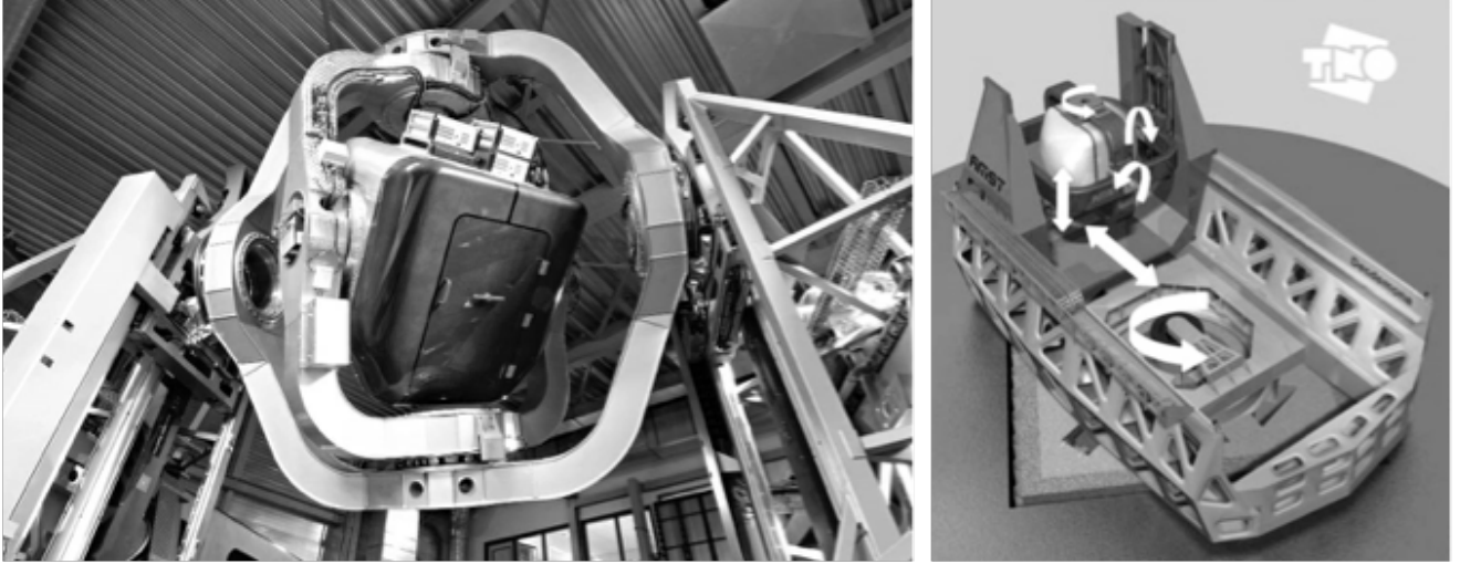
Fig. 4. The Desdemona simulator at TNO/Desdemona B.V. in Soesterberg, The Netherlands (Ref. 25).
