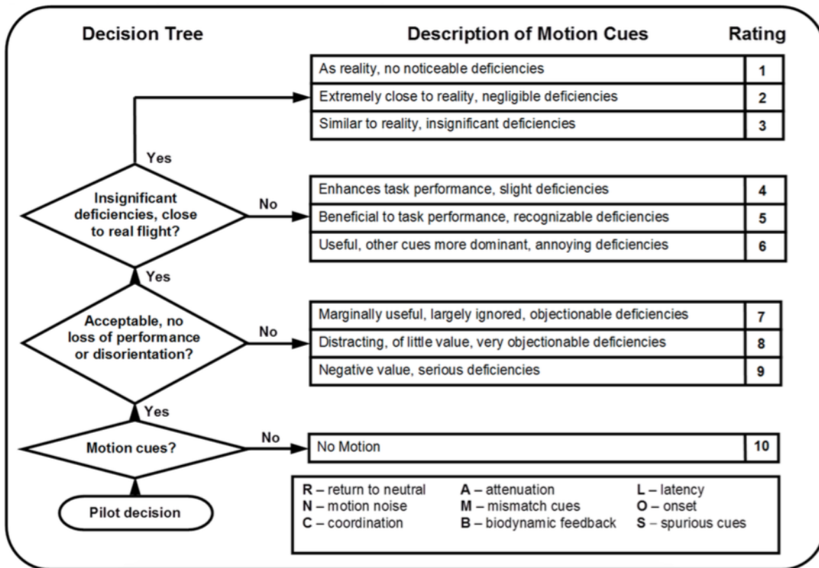
Fig. 3. The Motion Fidelity Rating (MFR) scale (Ref. 24).
