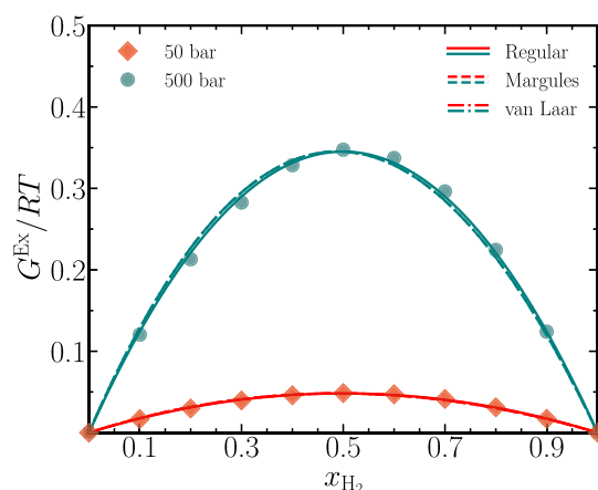
Figure 7. Gibbs-excess energies G^{Ex} in units of RT , where R is the universal gas constant, for binary mixtures of carbon dioxide and hydrogen, obtained from REFPROP 42 are plotted as symbols for p = 50 and 500 bar. Gibbs-excess energies derived from three different activity coefficient models, Regular, Margules, and van Laar, are fitted to the symbols. All data are reported at T = 323.15 K.
