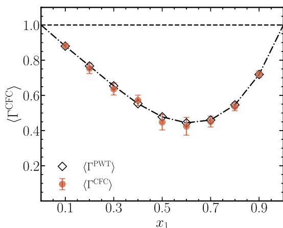
Figure 3. Comparison between the thermodynamic factors obtained using the CFCMC method ( \langle \Gamma^{\text{CFC}} \rangle ) (eq 25) and the PWTPI method ( \langle \Gamma^{\text{PWT}} \rangle ) 21 for a binary mixture of LJ molecules at a reduced temperature T = 2 and a reduced pressure of p = 2.8 . The reduced densities range between 0.4 at x_1 = 0.1 and 0.6 at x_1 = 0.9 . The black dashed-dotted line connecting the black diamond symbols is drawn to aid the eye.
