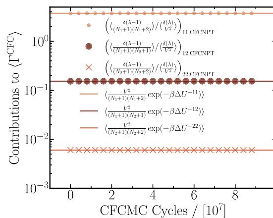
Figure 1. Individual terms (Table 1) from the CFCMC method, plotted as a function of the number of CFCMC production cycles for a binary mixture of LJ molecules simulated at a reduced temperature T = 2 , reduced pressure p = 2.8 , and x_1 = 0.1 . An average (reduced) density of \rho = 0.43 agrees well with the simulations from the PWTPM method. 21 Each data point is a block average over 40 independent CFCMC simulations. Lines represent mean values from the PWTPM method (eq 8) for the corresponding CFCMC terms. Terms related to single molecule insertions are omitted as these are canceled out by the Gibbs–Duhem equation (eq 26).
