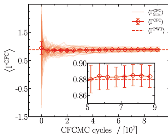
Figure 2. Evolution of \langle \Gamma^{\text{CFC}} \rangle with the number of CFCMC production cycles is plotted for a binary mixture of LJ molecules at T = 2 and p = 2.8 in reduced units and x_1 = 0.1 . Every symbol and the accompanying errors in measurement are computed by evaluating block-averages of \langle \Gamma^{\text{CFC}}_{\text{Sim}_i} \rangle from 40 independent simulations, where i corresponds to the number of the independent simulations. For comparison with the PWTPM method, \langle \Gamma^{\text{PWT}} \rangle is plotted as a dashed line. The inset zooms in on \langle \Gamma^{\text{CFC}} \rangle between 5 \times 10^7 and 9 \times 10^7 , while retaining \langle \Gamma^{\text{PWT}} \rangle for comparison.
