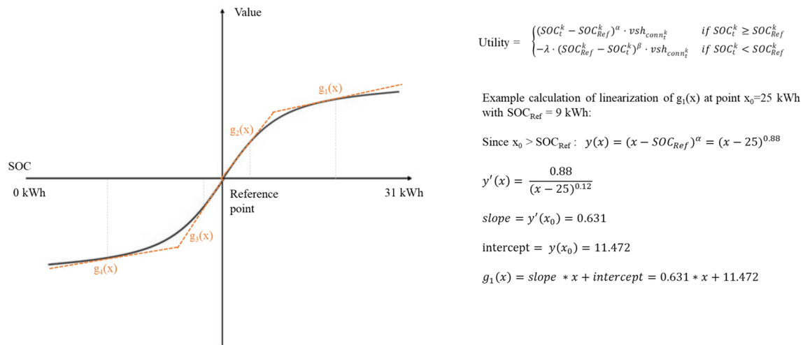
Fig. 6 Linear approximation of MINLP
