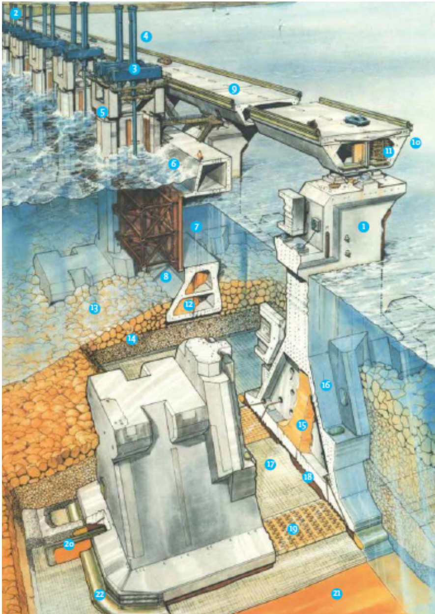
Figure 3: An overview of the Eastern Scheldt barrier's construction parts (right) and a cross section of its pillars (left). Source: Steenpoorte (2014), De stormvloedkering in de Oosterschelde .
