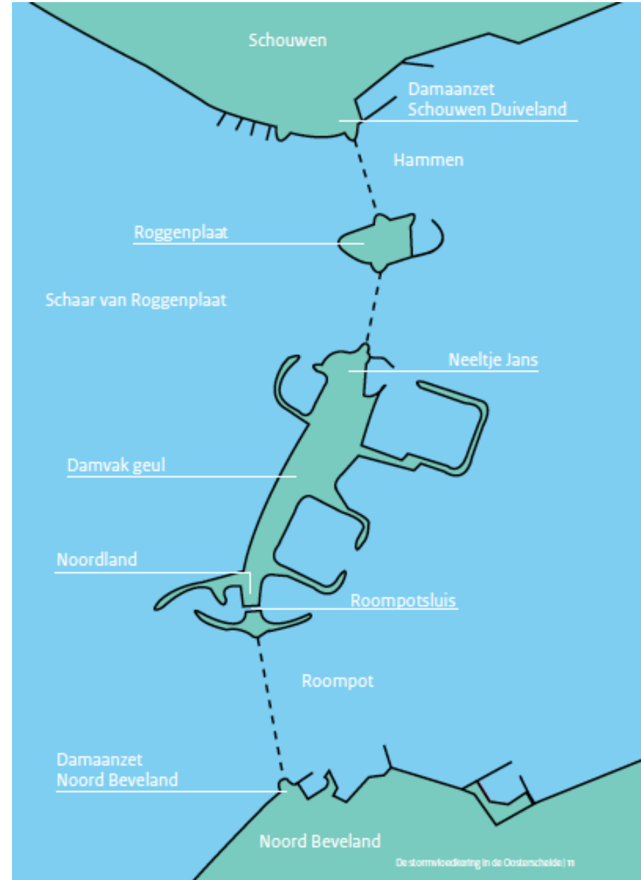
Figure 3: An overview of the Eastern Scheldt barrier's construction parts (right) and a cross section of its pillars (left). Source: Steenpoorte (2014), De stormvloedkering in de Oosterschelde .
