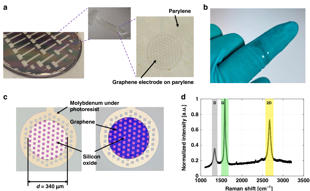
Fig. 2 Suspended multilayer graphene electrodes with different polymers (Parylene C and PDMS). a Suspended graphene electrodes with parylene-C substrate, b Suspended graphene electrode with PDMS substrate, c Optical image of the electrode before (yellow) and after (blue) Mo removal, d Raman Spectroscopy on graphene electrodes.
