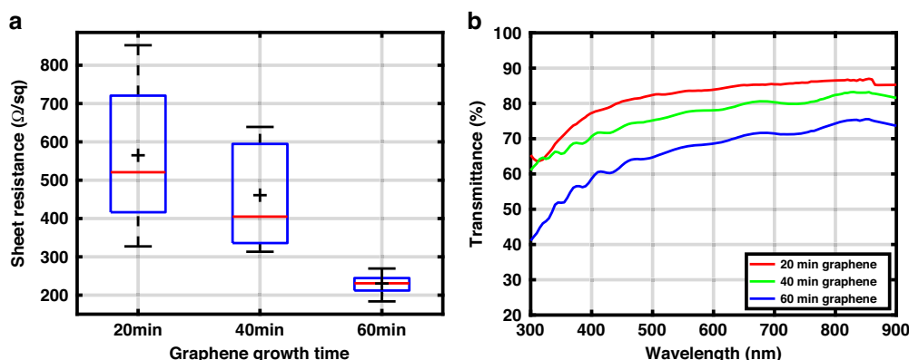
Fig. 3 Sheet resistance and optical transmittance characterization of graphene with different thicknesses. a Sheet resistance of three different graphene recipes (growth time: 20, 40, and 60 min) showing the maximum, upper quartile, median (red line), average (plus sign), lower quartile, and minimum values, b Optical transmittance measurements for different graphene growth times (the effect of the glass slide is removed).
