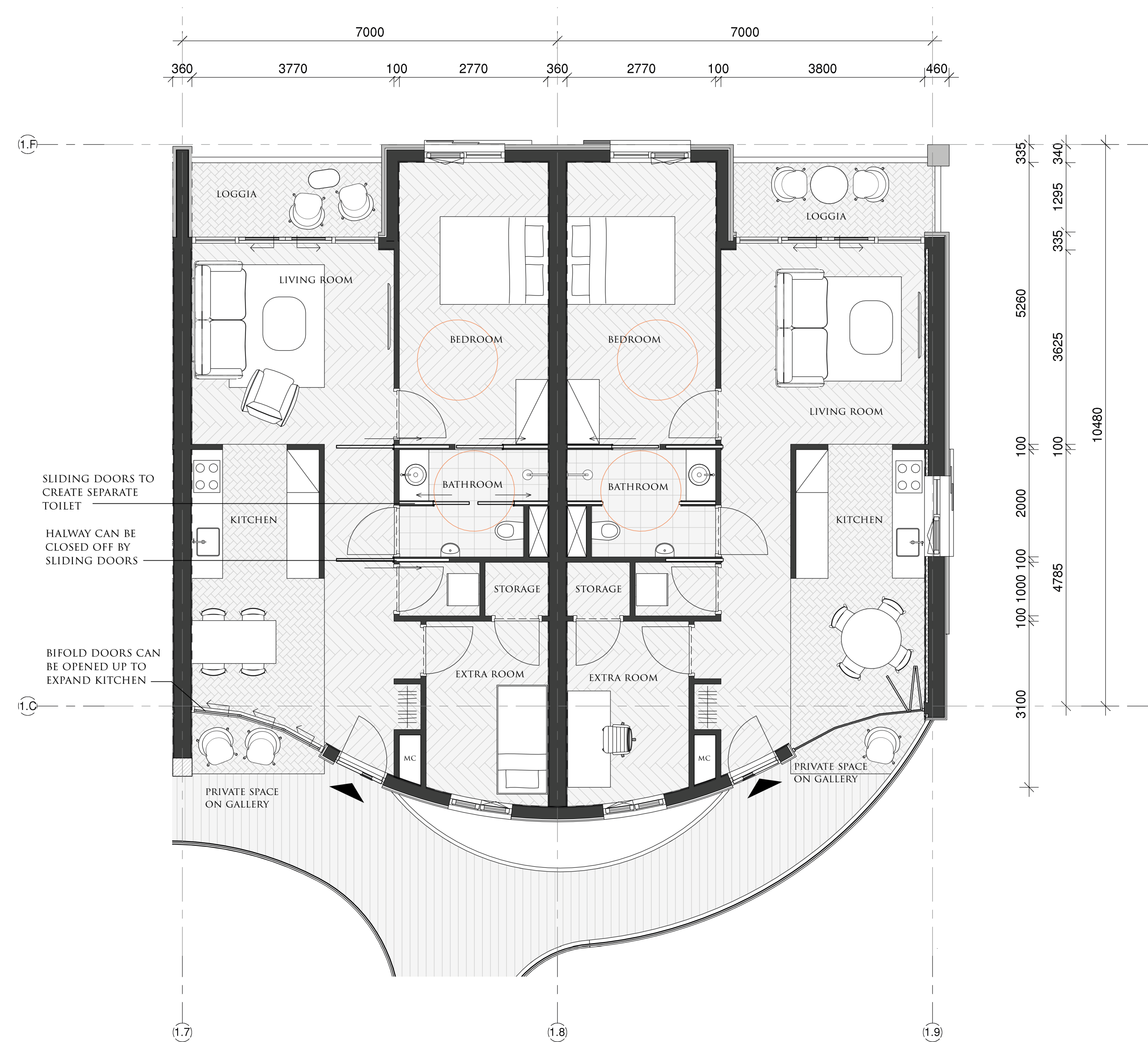
PLAN APARTMENT 1:50
