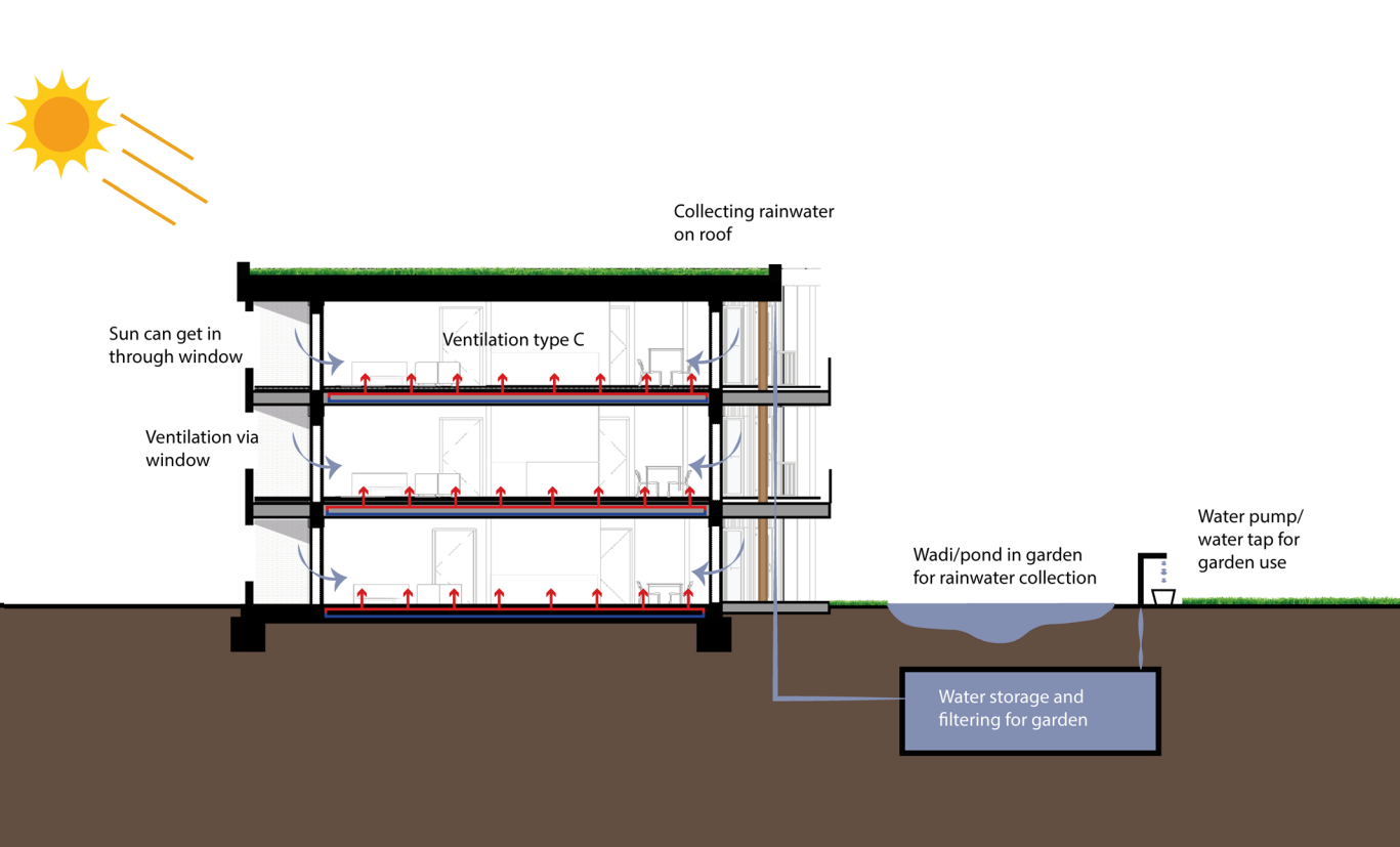
CLIMATE SECTION B WINTER
