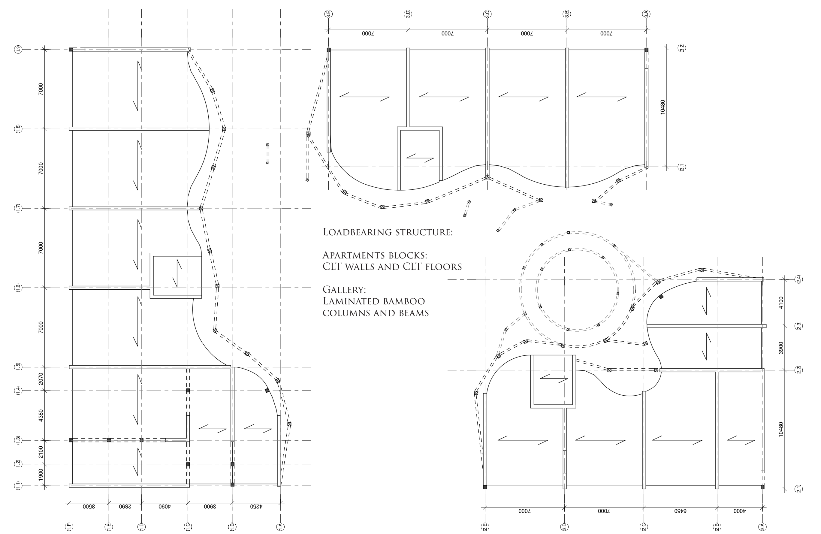
CONSTRUCTION PLAN GROUND FLOOR 1:200
