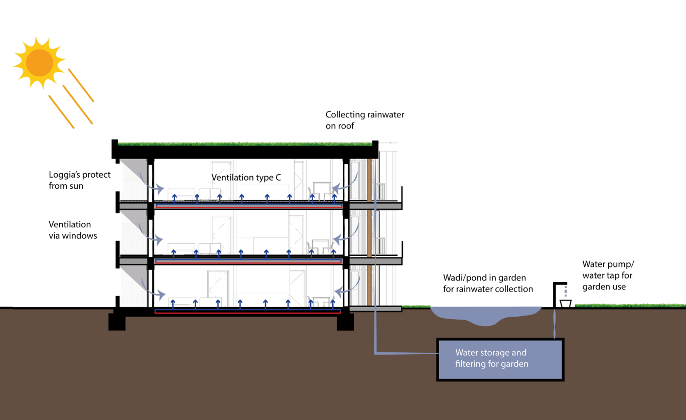
CLIMATE SECTION B SUMMER
