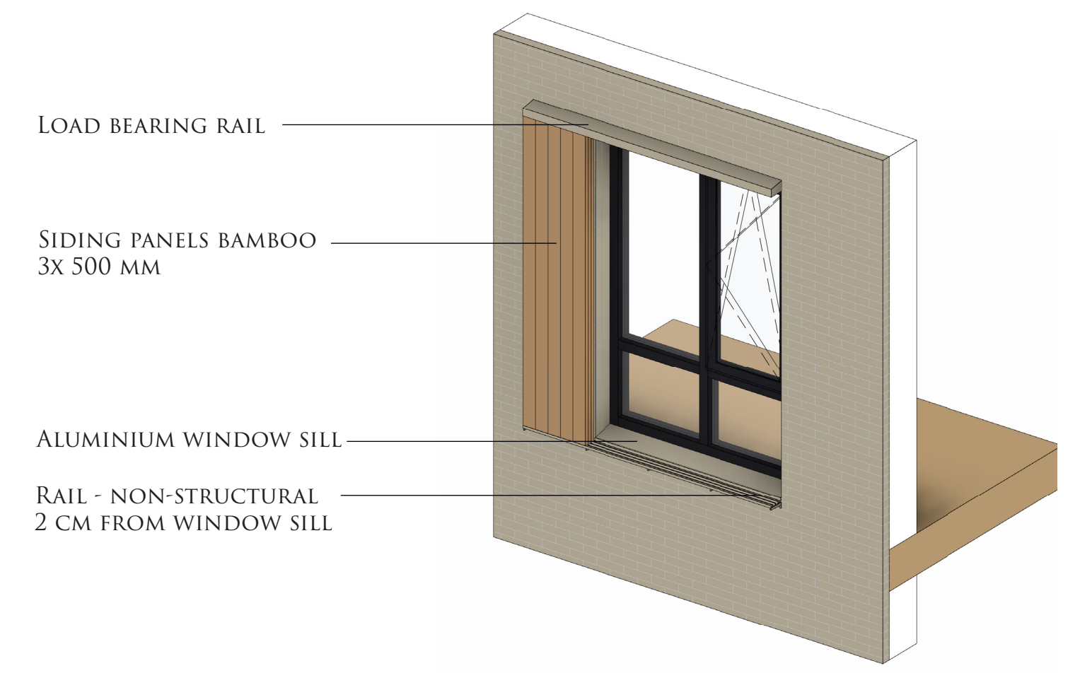
SLIDING PANELS FOR SUNSHADING OPEN
