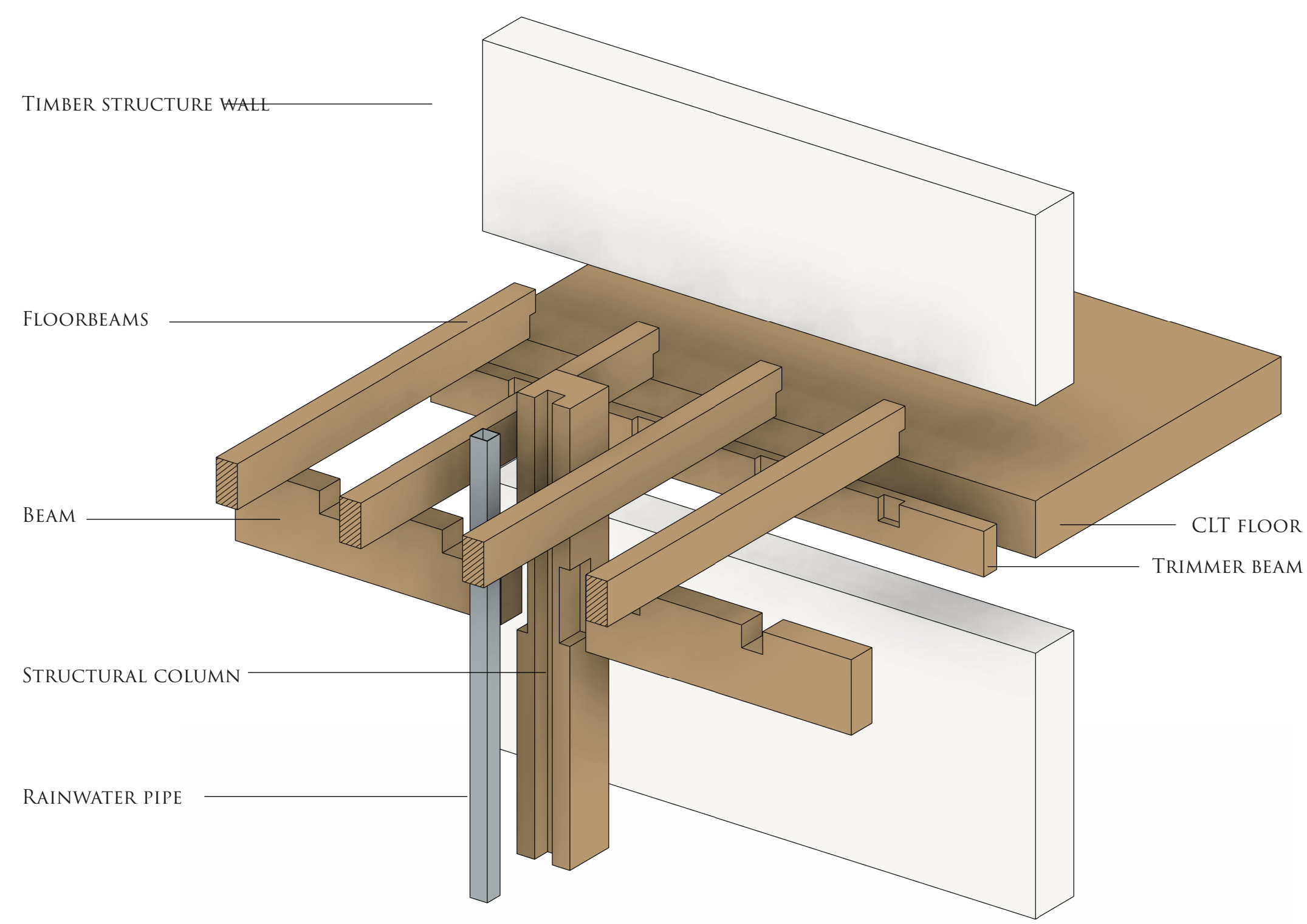
3D DETAIL CONSTRUCTION GALLERY
