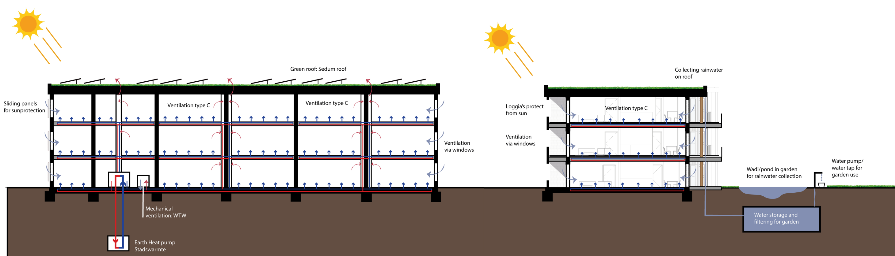
CLIMATE SECTION A SUMMER
