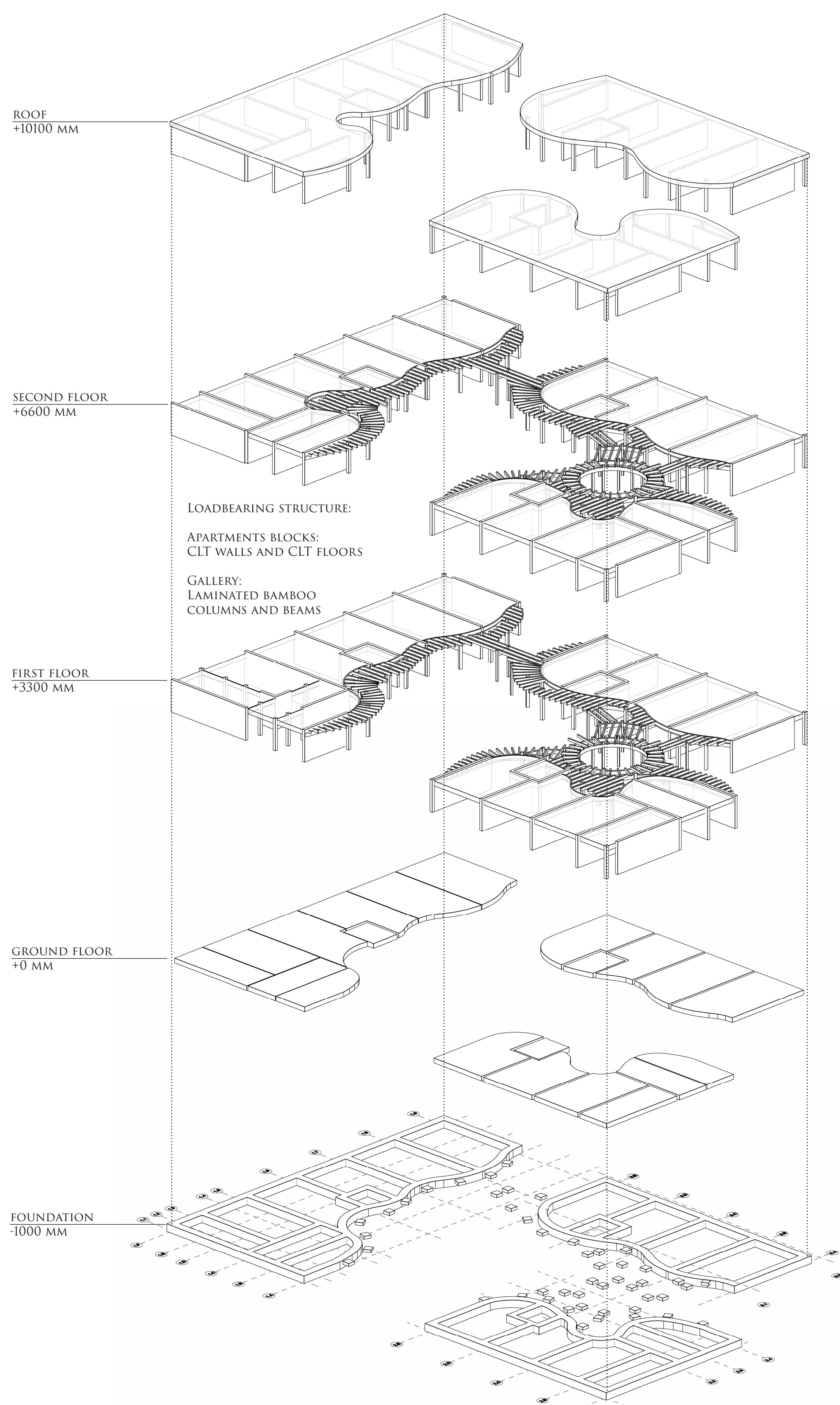
AXONOMETRY CONSTRUCTION
