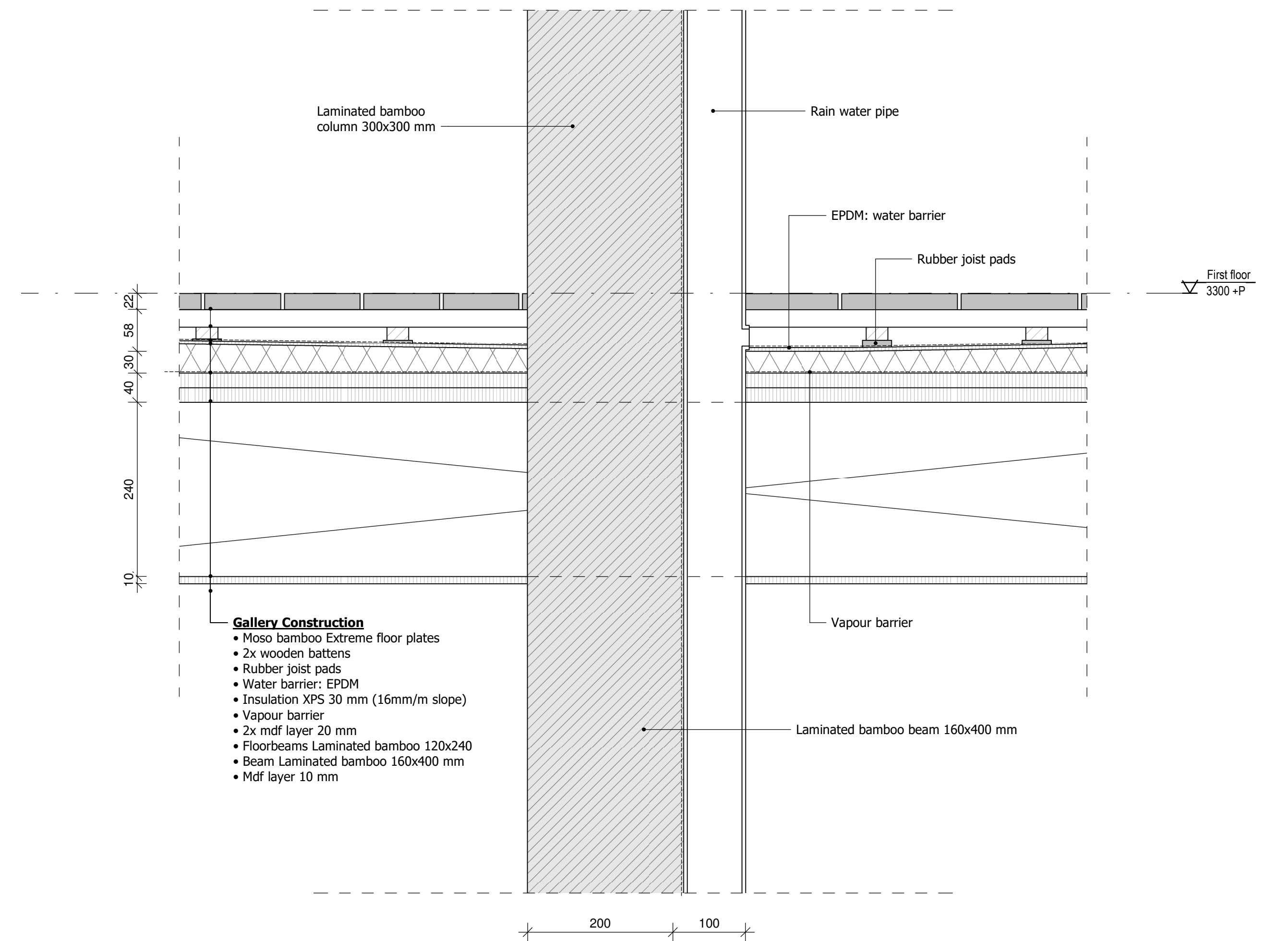
DETAIL B 1:5
