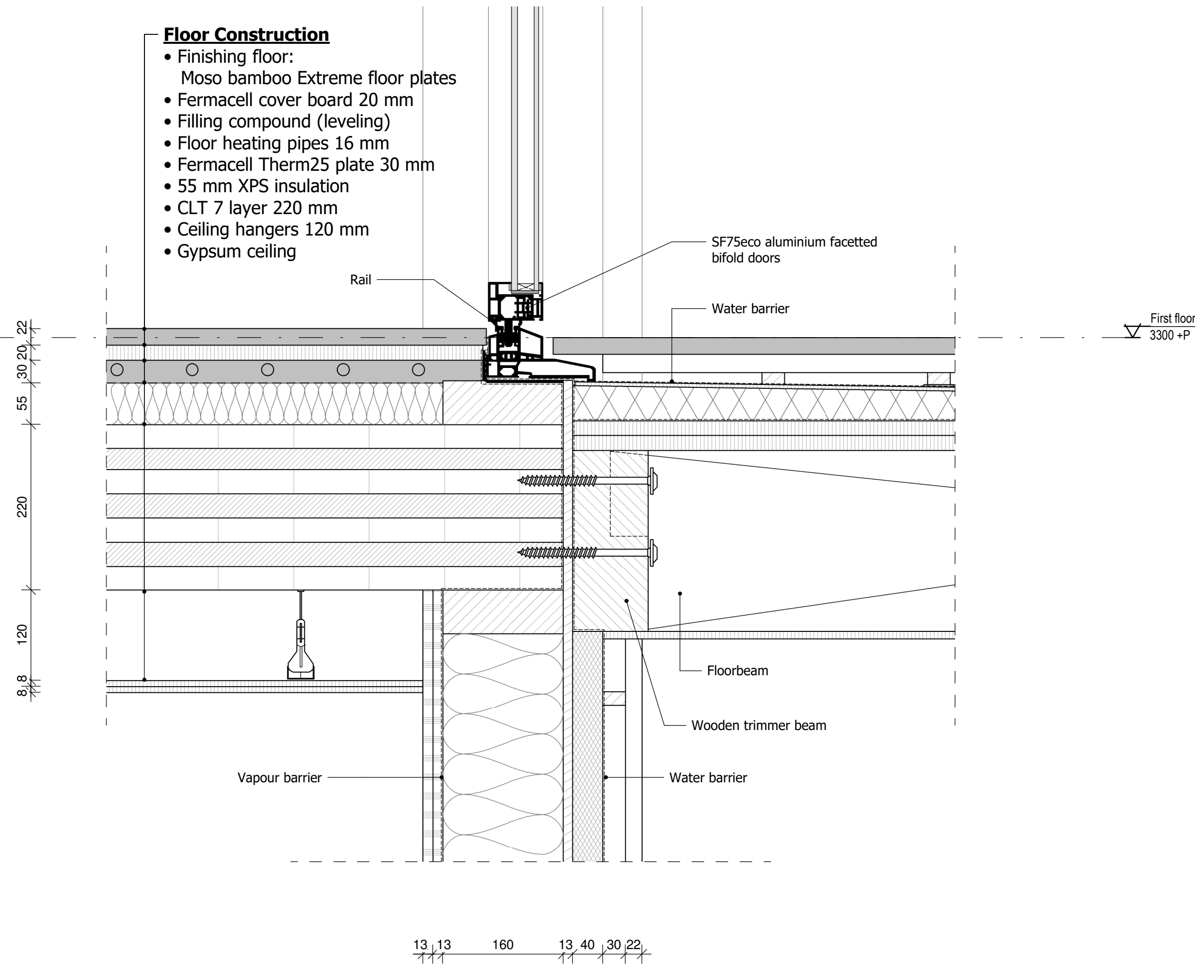
DETAIL A 1:5
