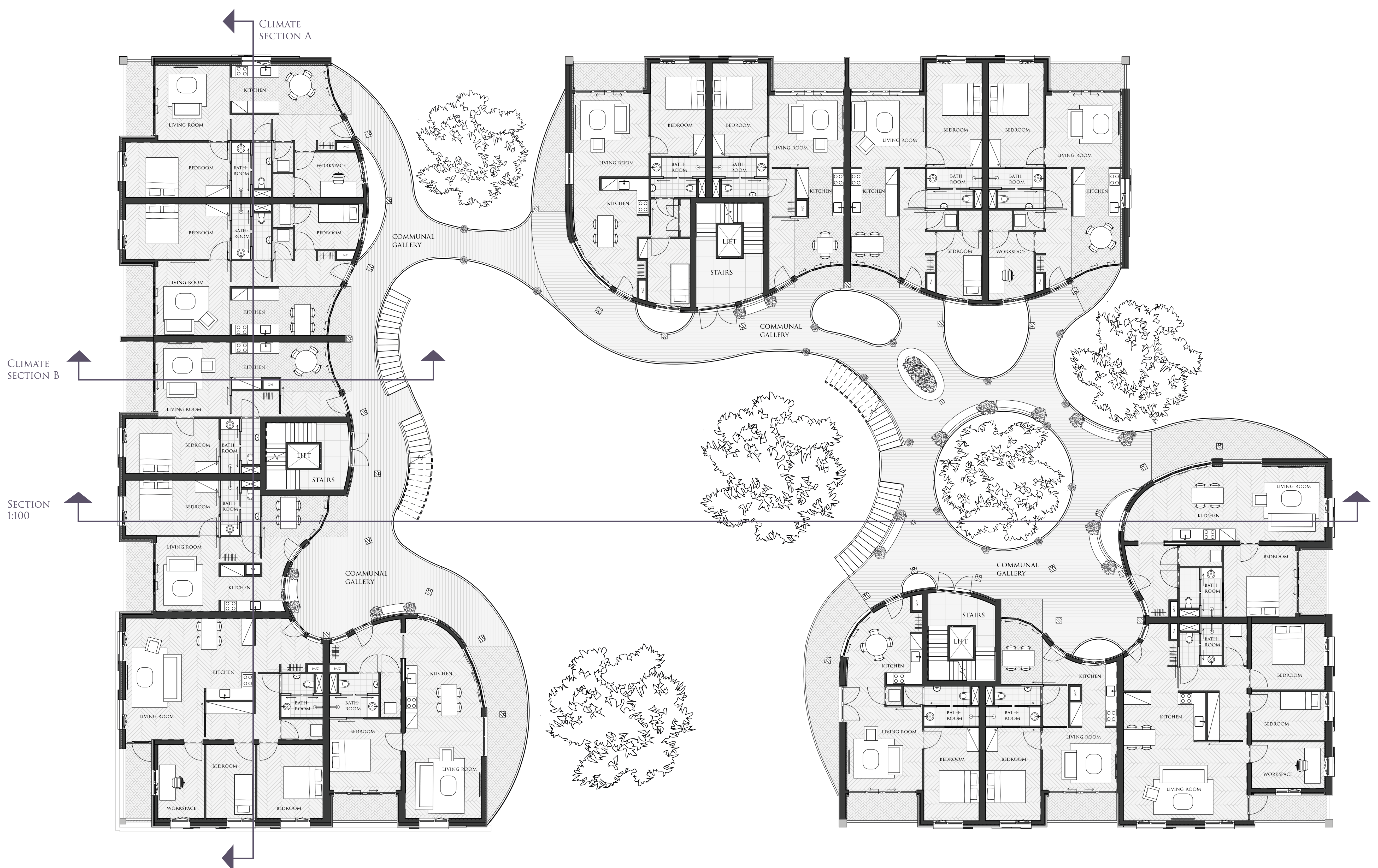
FIRST/SECOND FLOOR 1:100
