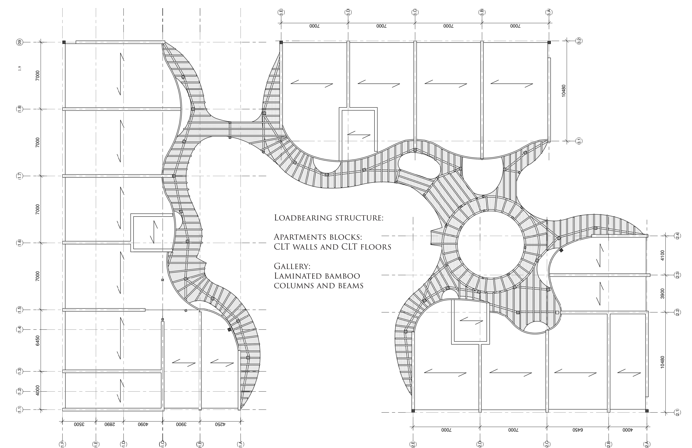
CONSTRUCTION PLAN FIRST/SECOND FLOOR 1:200
