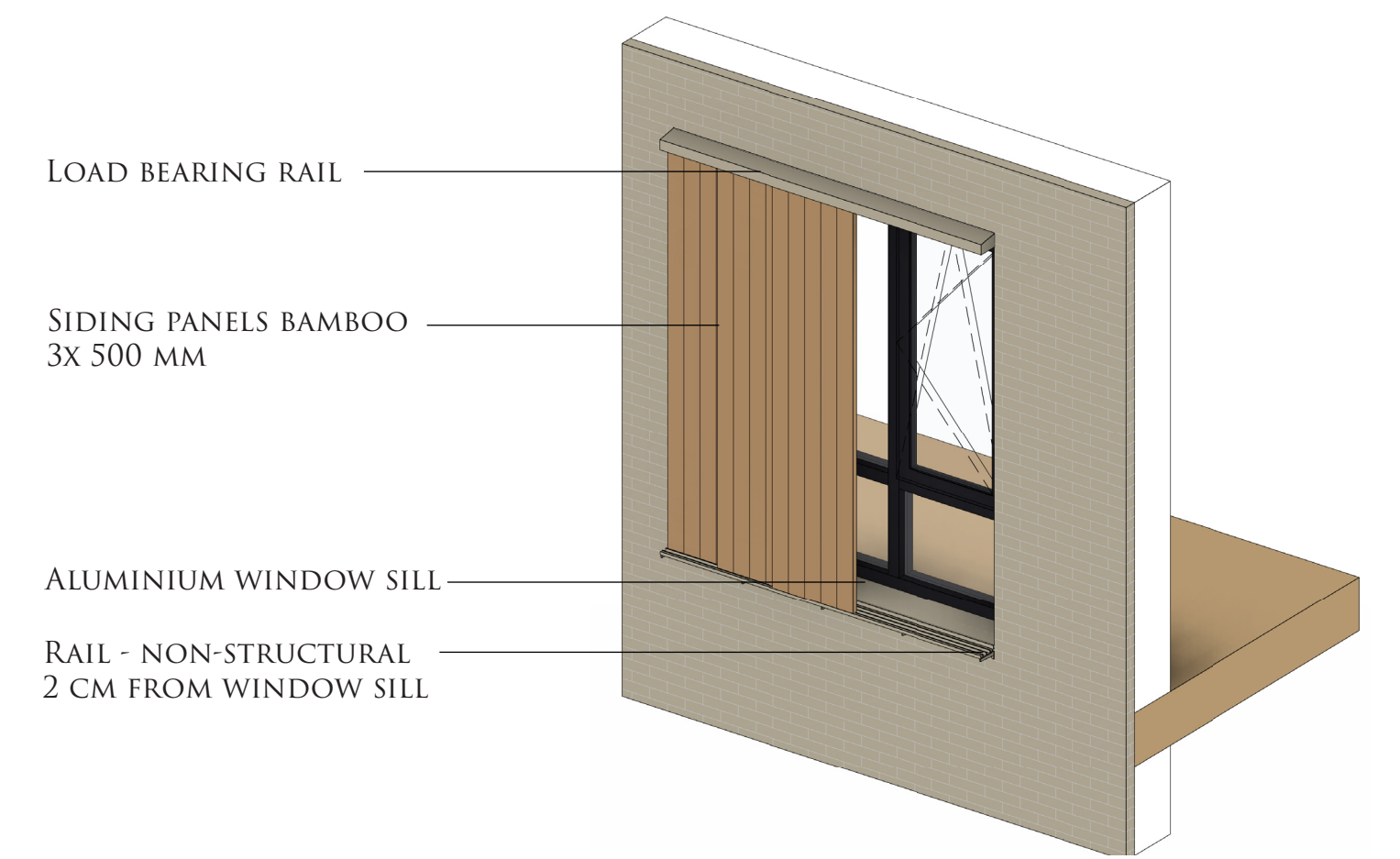
SLIDING PANELS FOR SUNSHADING CLOSED
