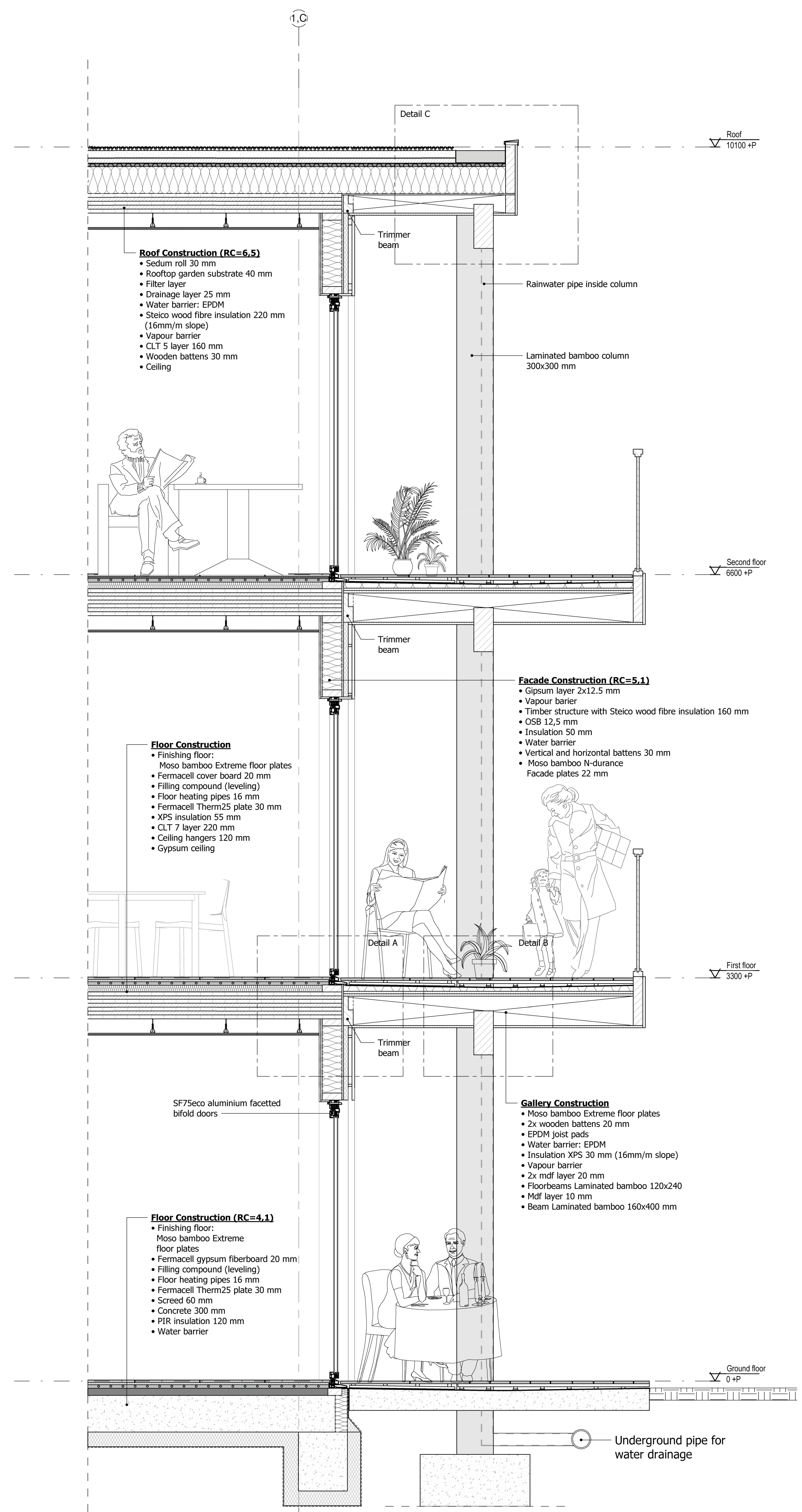
FACADE SECTION 1:20
