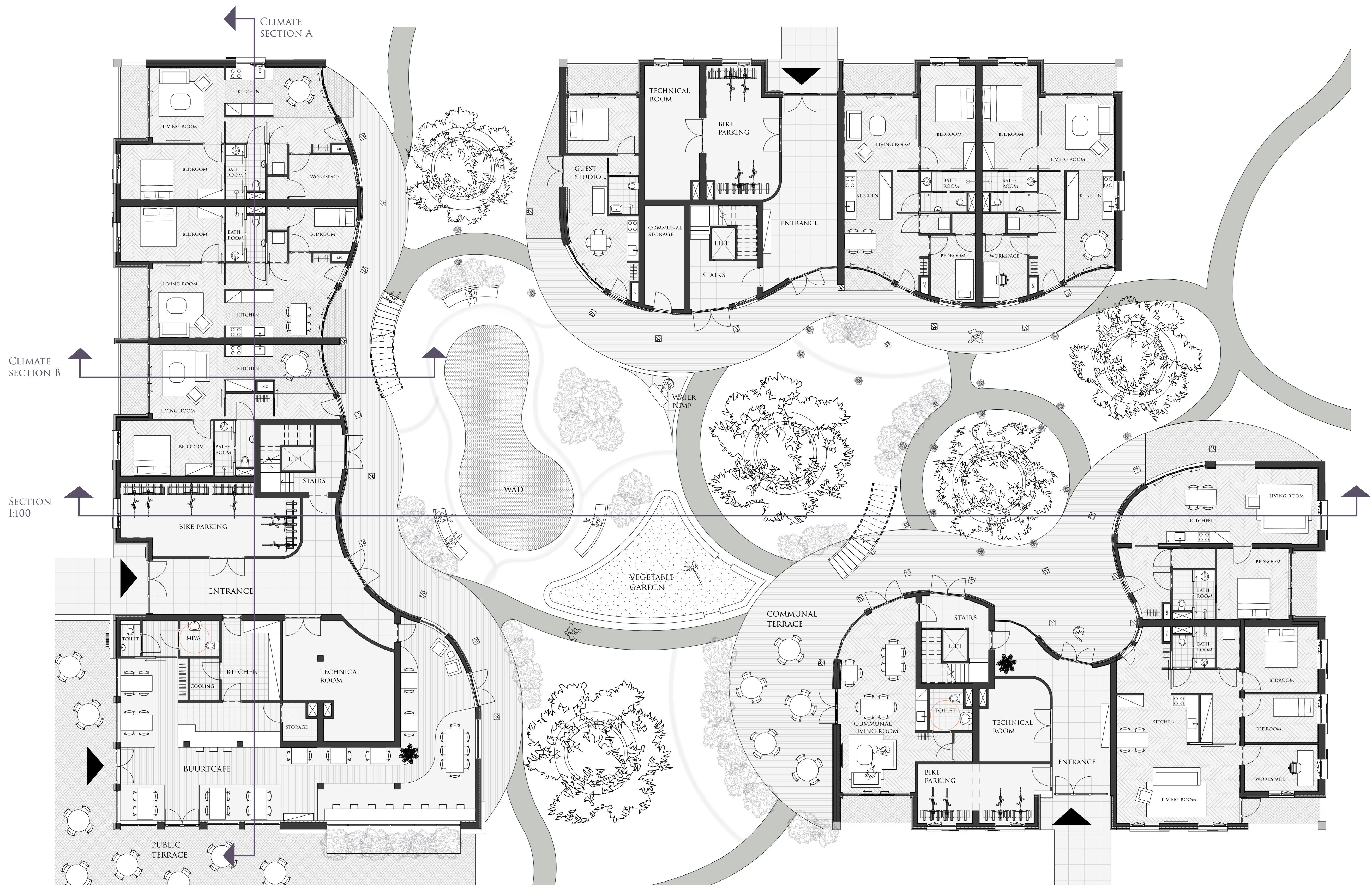
GROUND FLOOR 1:100
