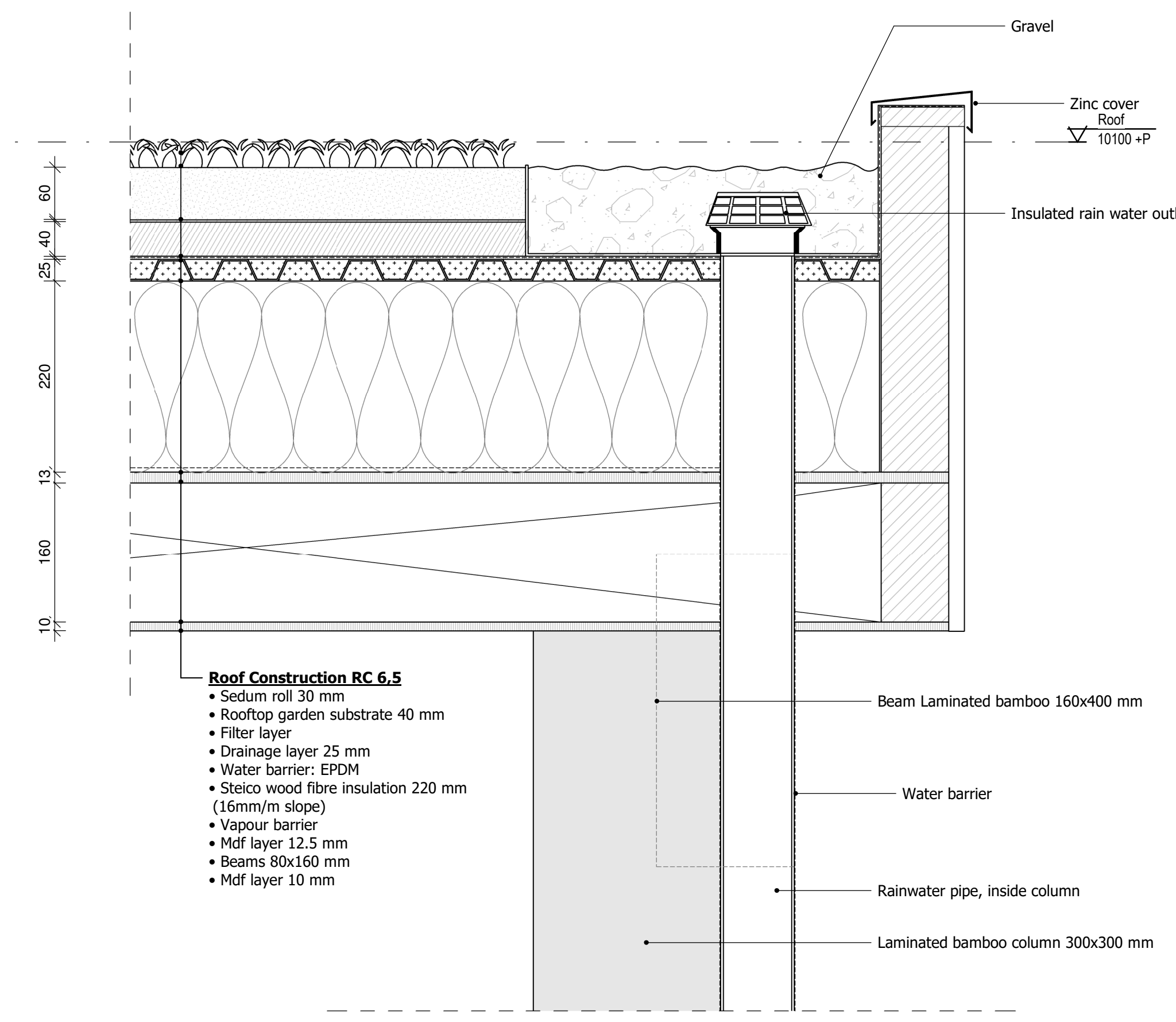
DETAIL C 1:5
