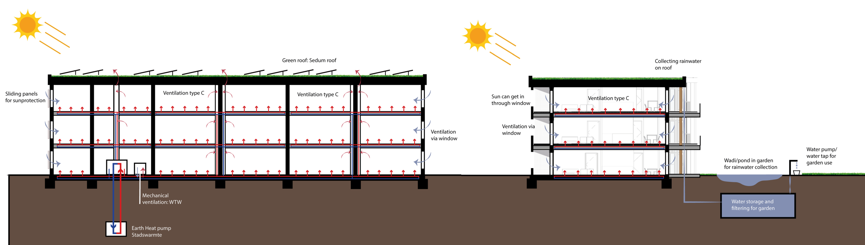
CLIMATE SECTION A WINTER
