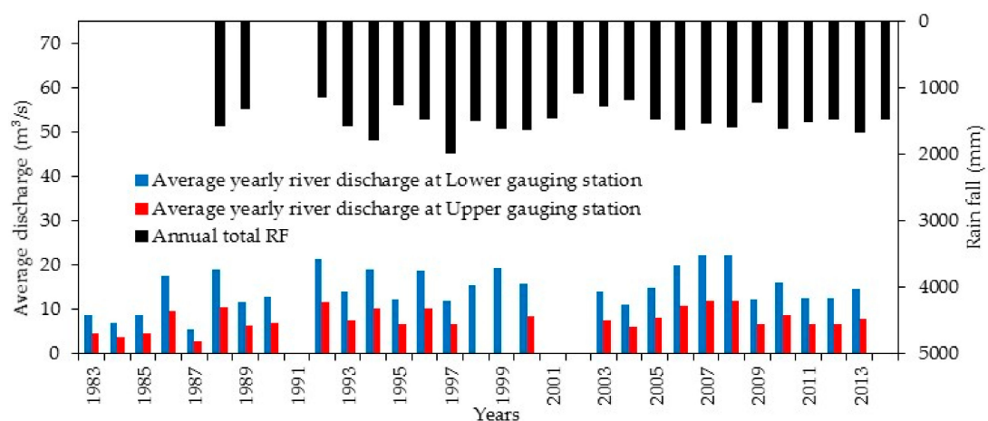
Figure 2. Yearly rainfall from the year 1988 to 2014 and average Ribb River discharges from the year 1983 to 2013 for the Lower and Upper gauging stations. The graph does not show any increasing or decreasing trends. Data source: National Meteorological Agency and Ministry of Water, Irrigation and Energy, Ethiopia.
