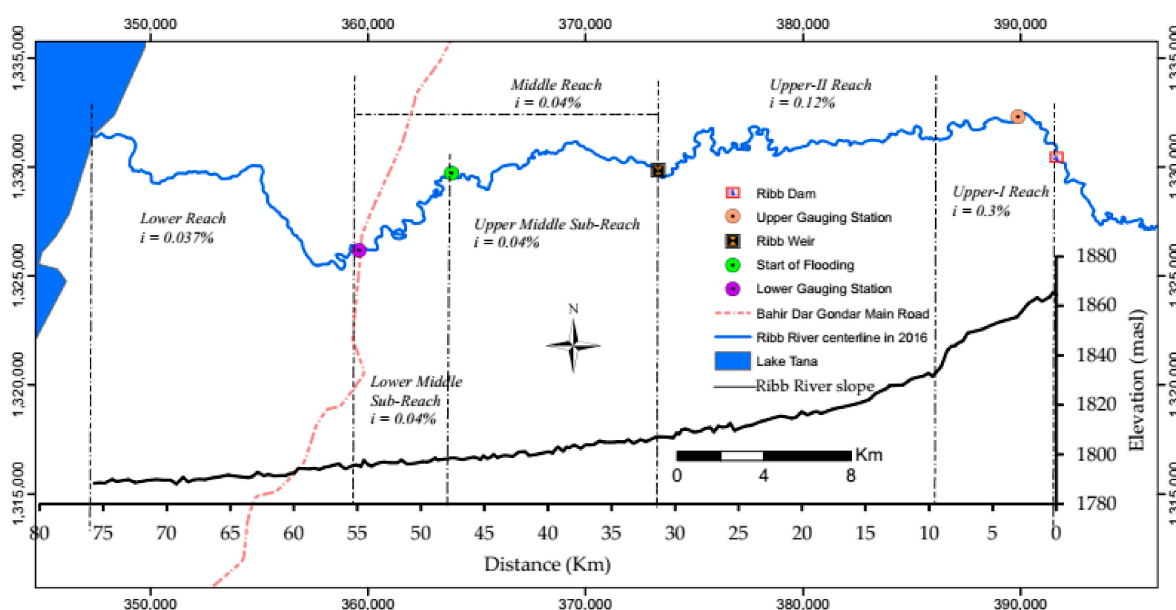
Figure 3. Ribb River study reach, sub-reaches and riverbed profile from the dam site to Lake Tana. The river alignment is derived from Google Earth images of 2016. The slope is obtained from 30 m resolution Digital Elevation Models (DEM) of Advanced Spaceborne Thermal Emission and Reflection Radiometer (ASTER) satellite images of 2014.
