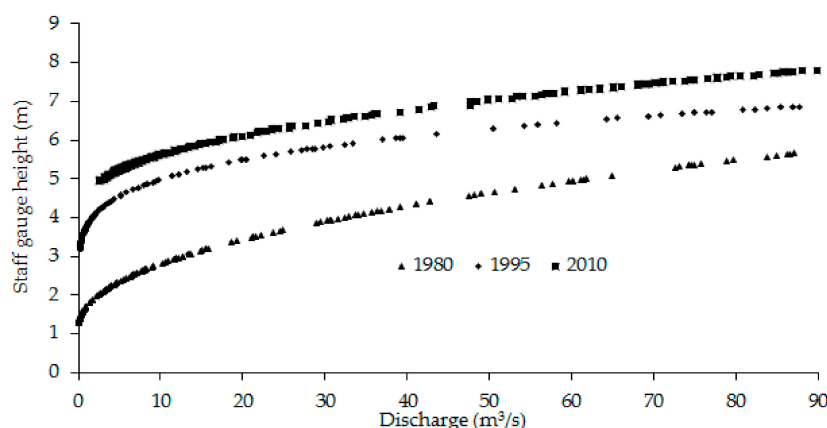
Figure 12. Ribb River staff level at the Lower gauging station with corresponding discharges (Data source: Ministry of Water, Irrigation and Energy, Ethiopia).
