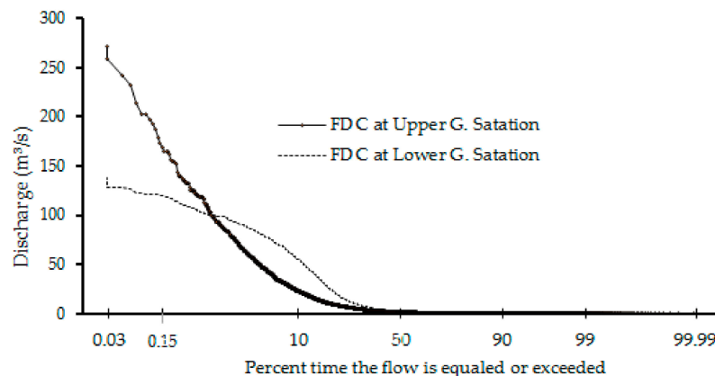
Figure 11. Flow duration curves at the Lower and Upper gauging stations (data source: Ministry of Water, Irrigation and Energy).
