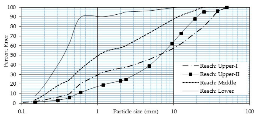
Figure 7. Grain size distribution of Ribb River bed material downstream of the Ribb Dam site, upstream and downstream of the weir site and upstream of the Ribb Bridge, at Universal Transverse Mercator (UTM) coordinates 37P 0388475, 1332080, 1872 m a.s.l.; 37P 0373692, 1329576, 1819 m a.s.l.; 37P 0368803, 1330762, 1804 m a.s.l. and 37P 0359808, 1326196, 1795 m a.s.l., respectively (Samples were collected in March 2016).
