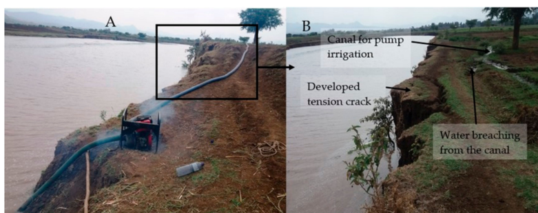
Figure 9. (A) water extraction with a diesel pump for irrigation; (B) irrigation canal to transport extracted water, which has been breached, and adjacent failing banks. The photos were taken immediately upstream of the under-construction Ribb weir in April 2017.
