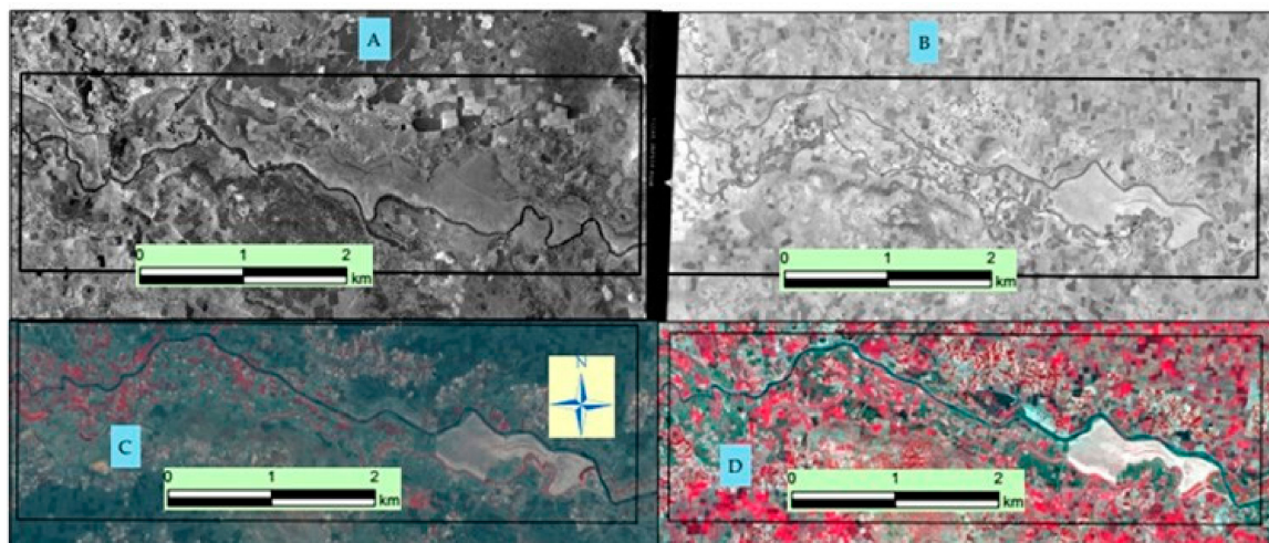
Figure 15. Aerial photographs and SPOT satellite images of the Middle river section downstream of the weir. (A,B) aerial photograph and river pattern of the year 1957 and 1980, respectively, and (C,D) SPOT satellite image and river pattern of the year 2006 and 2012, respectively.
