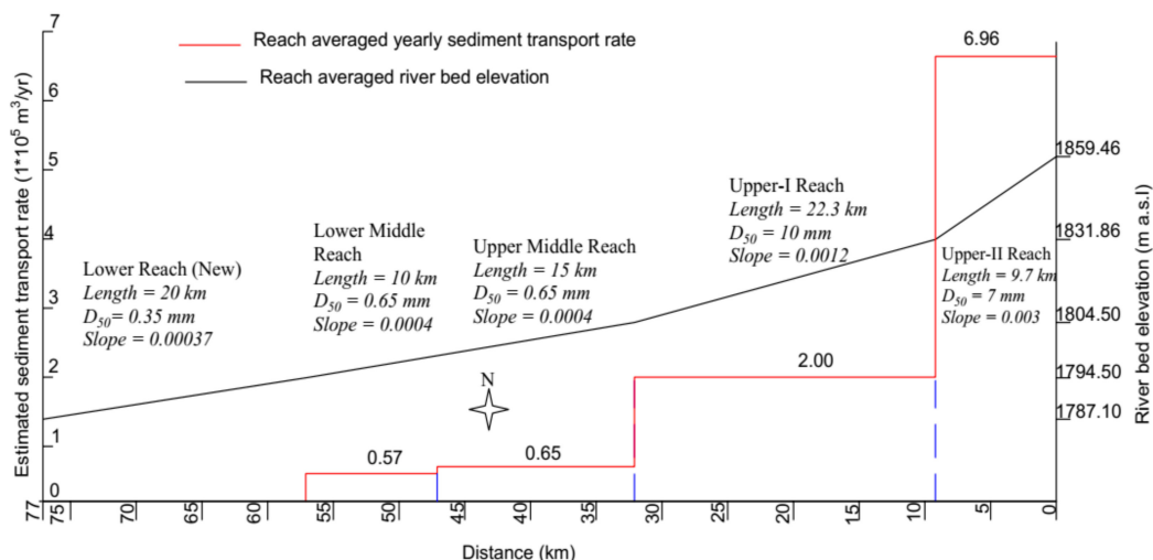
Figure 13. Sedimentation trend along the Ribb River based on estimated sediment transport rates. Distance of 0 km corresponds for dam site while 77 km is Lake Tana.
