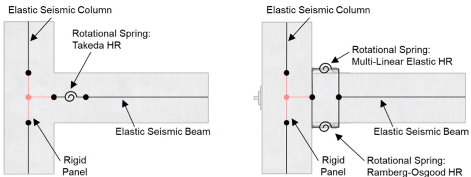
Fig. 11 Schematic representation of the lumped plasticity modelling approach adopted for the traditional (left) and low-damage (right) connections
