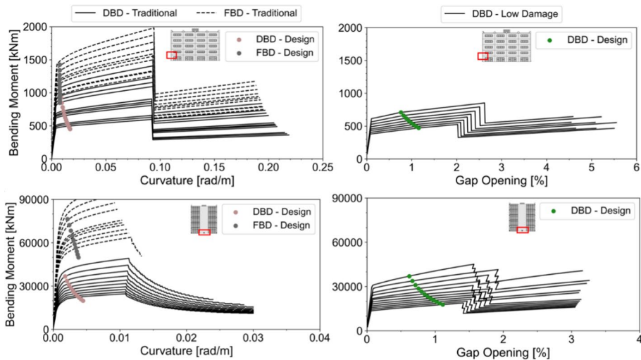
Fig. 10 Moment–curvature/rotation relationships of seismic beams (first floor) and structural walls for both Traditional buildings (left) and Low Damage buildings (right), for the case of high seismicity and Importance Class II
