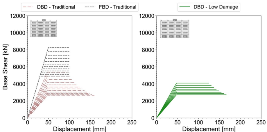
Fig. 8 Analytical capacity curves for the Traditional buildings (left) designed following FBD and DDBD procedures, and for the Low Damage buildings (right), in case of high seismicity and Importance Class II—frame direction only
