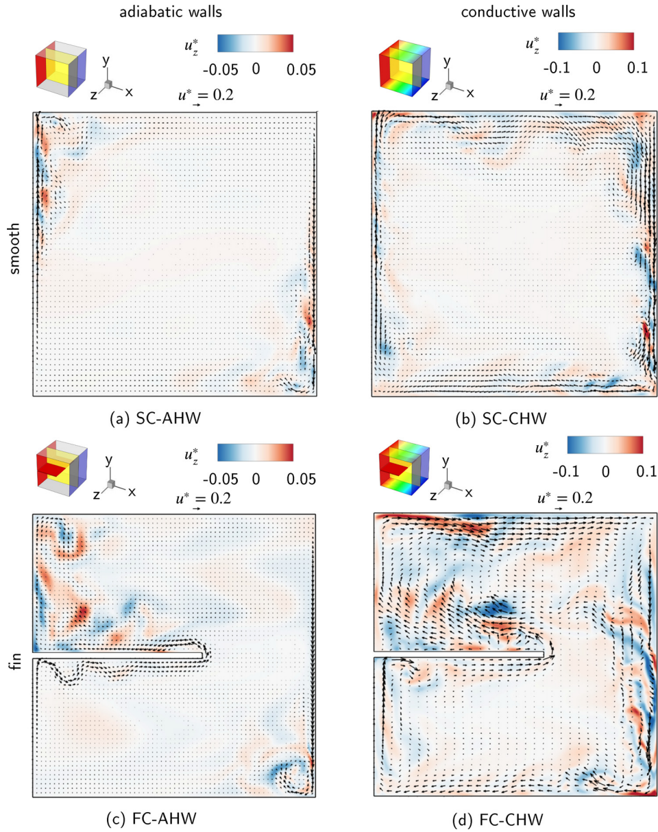
Fig. 6. Instantaneous 2D vector field of the in-plane velocity (i.e., in x-and y-direction) and contour map of out-of-plane velocity (i.e., the velocity in z-direction) for Ra = 10^9 . Note that to improve the quality of presentation, results obtained on the original non-uniform mesh are mapped onto a uniform mesh of size. The velocities are scaled with the buoyancy velocity U_b for the corresponding Rayleigh number. Values outside the range u_z^* \in [-0.1, 0.1] are clipped. The geometry and thermal boundary conditions are illustrated by sketches in the top-left corner of each subfigure.
