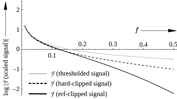
Figure 2: The Fourier transform of the signals after thresholding, hard-clipping and erf-clipping. The erf-clipping result corresponds to a Gaussian filtered step edge. The size of the Gaussian filters is similar to the size of the PSF, \sigma_{psf} = 0.9 .
