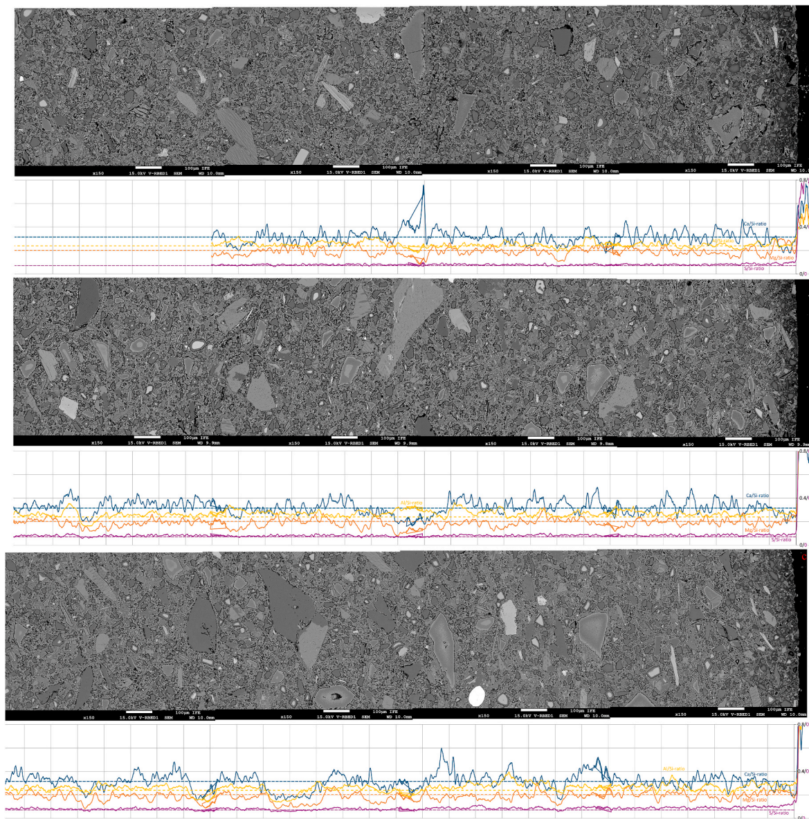
Fig. 23. SEM Micrographs of S5 samples exposed to wet supercritical CO 2 equilibrated with concentrated H 2 SO 4 for 4 (a), 8 (b), and 16 (c) weeks. The graphs underneath each micrograph show the Ca/Si, Mg/Si and Al/Si (blue, orange and yellow, respectively, all on the 0–0.8 axis), and S/Si (purple, on the 0–0.4 axis) elemental ratios (atom %/atom %) measured along the micrograph using EDS. The dashed lines are reference values (average values) measured at the centre of an unexposed sample. Scalebars shown with the micrographs and gridline spacing for the graphs are 100 \mu m.
