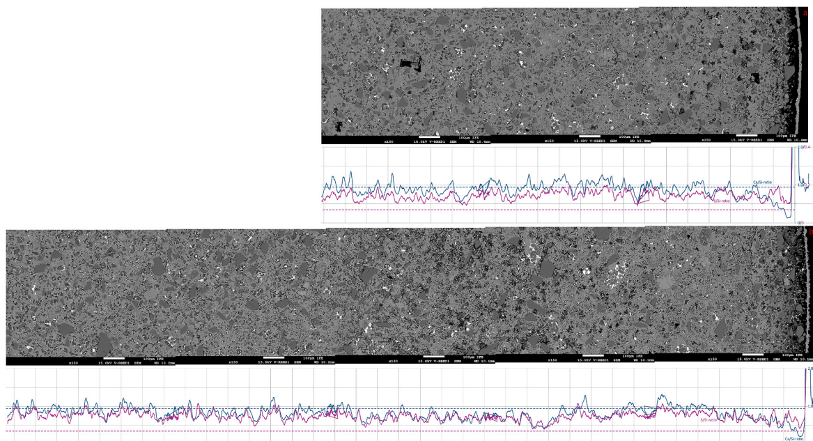
Fig. 9. SEM Micrographs of S2 samples exposed to water saturated with CO 2 containing 1.6 mol% H 2 S for 4 (a) and 16 (b) weeks. The graphs underneath each micrograph show the Ca/Si (blue, on the 0–2.0 axis) and S/Si (purple, on the 0–0.4 axis) elemental ratios (atom %/atom %) measured along the micrograph using EDS. The dashed lines are reference values (average values) measured at the centre of an unexposed sample. Scalebars shown with the micrographs and gridline spacing for the graphs are 100 µm.
