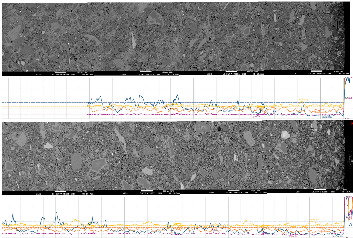
Fig. 21. SEM Micrographs of S5 samples exposed to water saturated with CO 2 containing 1.6 mol% H 2 S for 4 (a) and 16 (b) weeks. The graphs underneath each micrograph show the Ca/Si, Mg/Si and Al/Si (blue, orange and yellow, respectively, all on the 0–0.8 axis), and S/Si (purple, on the 0–0.4 axis) elemental ratios (atom %/atom %) measured along the micrograph using EDS. The dashed lines are reference values (average values) measured at the centre of an unexposed sample. Scalebars shown with the micrographs and gridline spacing for the graphs are 100 µm.
