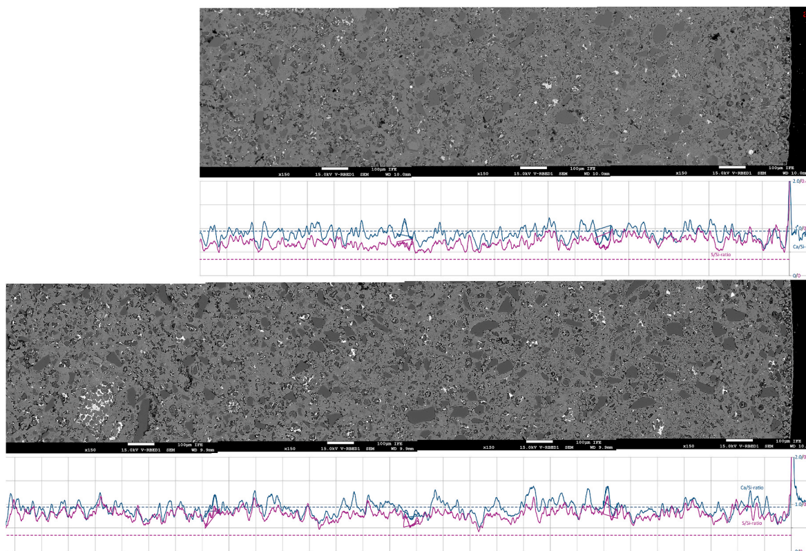
Fig. 10. SEM Micrographs of S2 samples exposed to wet supercritical CO 2 with 1.6 mol% H 2 S for 4 (a) and 16 (b) weeks. The graphs underneath each micrograph show the Ca/Si (blue, on the 0–2.0 axis) and S/Si (purple, on the 0–0.4 axis) elemental ratios (atom %/atom %) measured along the micrograph using EDS. The dashed lines are reference values (average values) measured at the centre of an unexposed sample. Scalebars shown with the micrographs and gridline spacing for the graphs are 100 µm.
