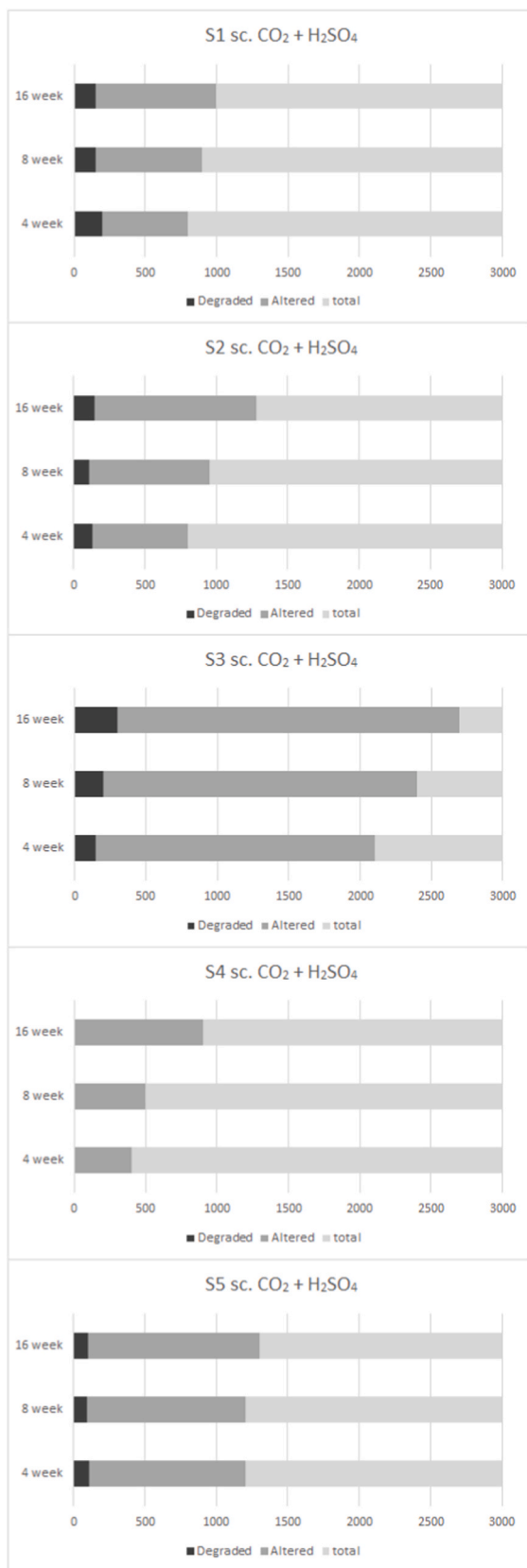
Fig. 25. Bar diagrams indicating the depths of degradation and the depth to which sealants were altered by exposure to CO 2 with H 2 SO 4 based on SEM micrographs, elemental ratios, and CT scanning.
