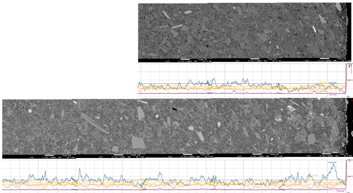
Fig. 22. SEM Micrographs of S5 samples exposed to wet supercritical CO 2 with 1.6 mol% H 2 S for 4 (a) and 16 (b) weeks. The graphs underneath each micrograph show the Ca/Si, Mg/Si and Al/Si (blue, orange and yellow, respectively, all on the 0–0.8 axis), and S/Si (purple, on the 0–0.4 axis) elemental ratios (atom %/atom %) measured along the micrograph using EDS. The dashed lines are reference values (average values) measured at the centre of an unexposed sample. Scalebars shown with the micrographs and gridline spacing for the graphs are 100 µm.
