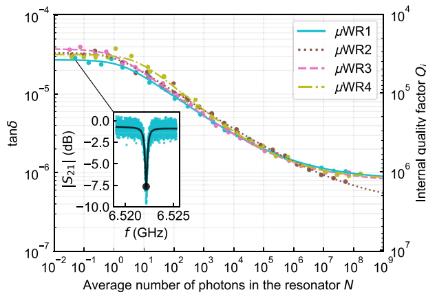
FIG. 9. Measured microwave \tan \delta = 1/(pQ_i) versus average number of photons in the resonators \mu\text{WR1-4} of chip 3. The curves are fits to Eq. (3). The inset illustrates how \tan \delta is obtained at each power, by fitting the |S_{21}| dips using the model in Ref. [36]. The \tan \delta_0 values are obtained by fitting the \tan \delta versus N curves to Eq. (3).
