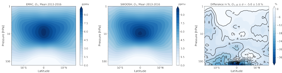
Figure A.2: Multi-annual mean (2013-2016) of \text{O}_3 volume mixing ratios for the EMAC setup RC1SD-base-10 (left), SWOOSH satellite data (middle) and the difference (observation-model) in percent (right).
