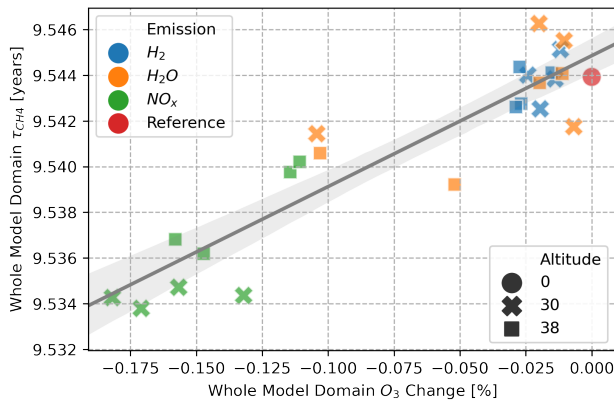
Figure A.33: Methane lifetime in relation to ozone change (both whole-model-domain) for all emission scenarios (legend). The gray regression line including the shaded area depict the 95 % confidence interval of all scenarios.
