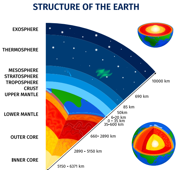
Figure 2.2: The layers from the Earth's core to the top of the atmosphere. The distance is not drawn to scale. Designed by freepik
