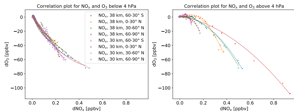
Figure A.24: Correlation of nitrogen oxide change and ozone change for two altitudes regions (surface-4 hPa and 4-0.01 hPa). The values are averaged over latitude and limited to statistically significant values with a 95 % confidence.
