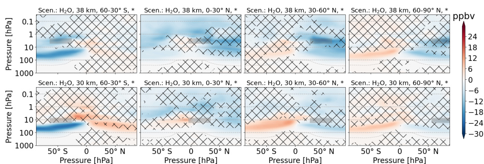
Figure 7.4: Zonal mean of CH_4 perturbation (volume mixing ratio, ppbv) for scenarios where H_2O is emitted. The first and second row refer to 38 km and 30 km altitudes of emission, respectively. Columns represent the latitude region of emission. The emission regions are shaded in gray. Lines indicate statistically insignificant results and the probability level is written in the title of each subplot.
