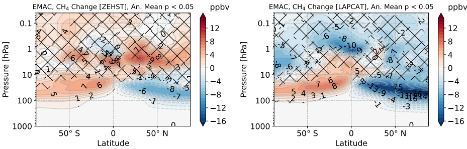
Figure 6.5: Multi-annual mean (2010-2014) of CH 4 perturbation (ppbv) for the ZEHST scenario (left) and the LAPCAT scenario (right) for EMAC. Hatched areas are characterized by a p-value higher than the threshold indicated in the title of each plot.
