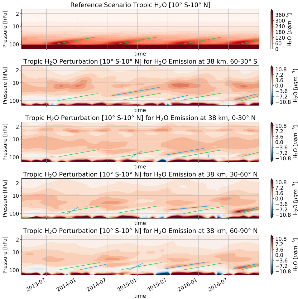
Figure 5.1: Timeline of integrated concentrations changes in the tropics ( 10^\circ S- 10^\circ N) for water vapor emission scenarios at 38 km altitude and the reference simulation (first row). Theoretical position of tape recorder features were marked with green lines and potential similar features in the perturbation scenarios were marked with blue lines.
