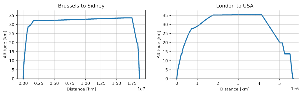
Figure 8.3: Altitude versus distance of trajectories between two city-pairs Brussels-Sidney (left) and London-New York (right).
