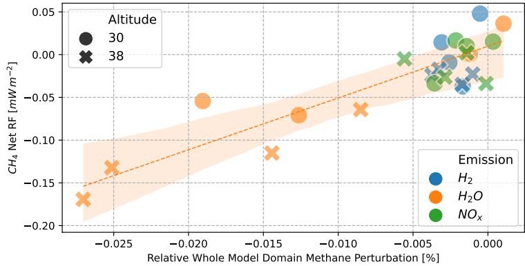
Figure 7.19: Overview of CH 4 net radiative forcing for all 24 simulations. Colors refer to the initial emission (H 2 , H 2 O and NO x ) and markers to altitudes of emission. The regression line including the shaded areas depict the mean and standard deviation of the eight H 2 O emission scenarios.
