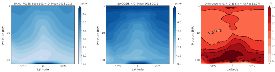
Figure A.1: Multi-annual mean (2013-2016) of \text{H}_2\text{O} volume mixing ratios for the EMAC setup RC1SD-base-10 (left), SWOOSH satellite data (middle) and the difference (observation-model) in percent (right).
