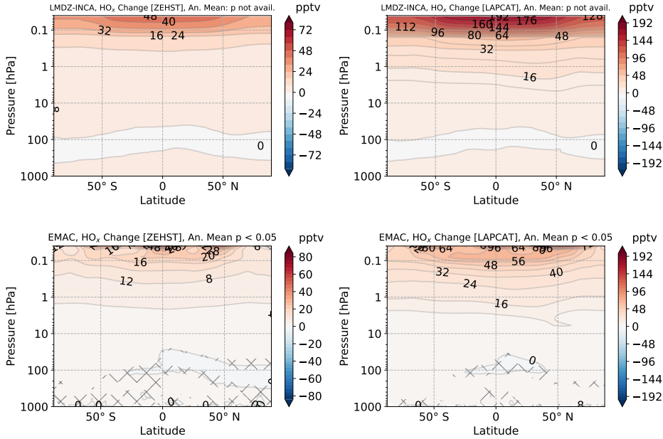
Figure A.12: Annual mean (2010-2014) of \text{HO}_x ( \text{OH} + \text{HO}_2 + \text{H} ) perturbation (pptv) for the ZEHST scenario (left) and the LAPCAT scenario (right) for EMAC (lower) and LMDZ-INCA (upper). hatched areas are characterized by a p-value higher than the threshold indicated in the title of each plot.
