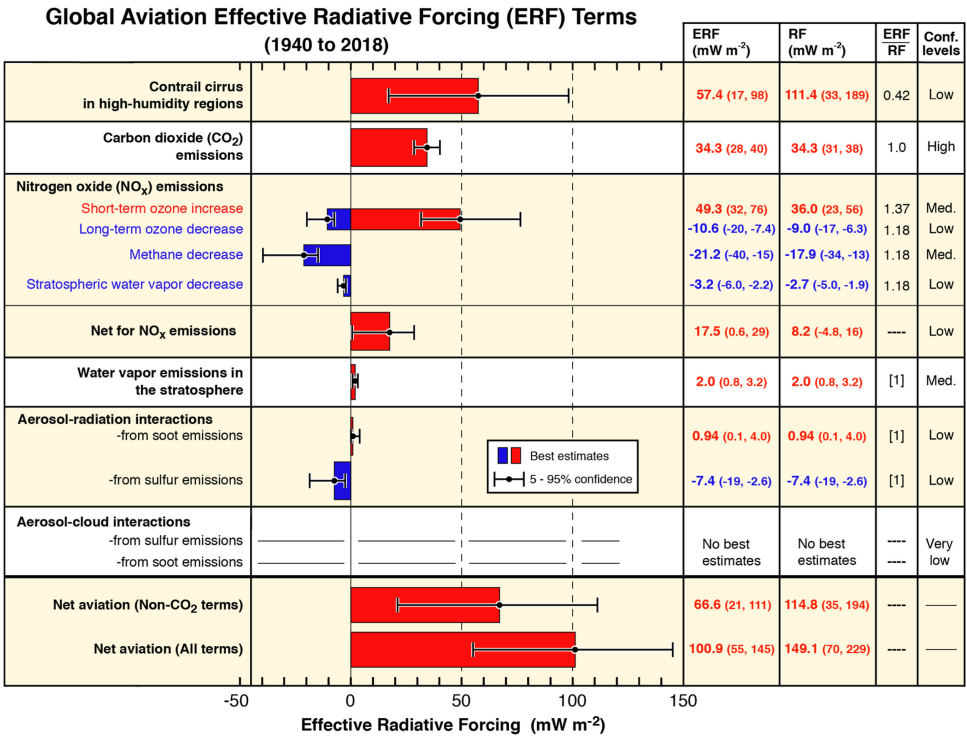
Figure 2.17: Best-estimates for climate forcing terms from global aviation from 1940 to 2018. The bars and whiskers show ERF, best estimates and the 5–95 % confidence intervals, respectively. Red bars indicate warming terms and blue bars indicate cooling terms. Numerical ERF and RF values are given in the columns with 5–95 % confidence intervals along with ERF/RF ratios and confidence levels. The figure and caption were reprinted from Lee et al. [5] with permission from Elsevier through RightsLink.
