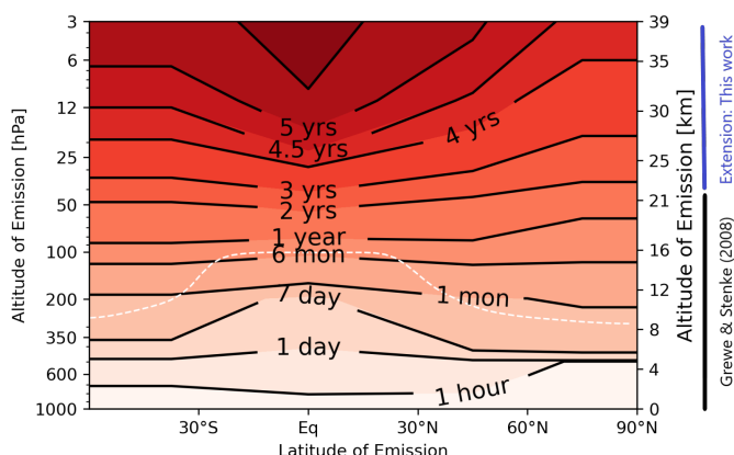
Figure 7.9: Reproduced from Grewe and Stenke [21], Fig. 6 (a), with permission from the authors, who provided the data. The figure shows the water vapor perturbation lifetime for the original pressure levels (1000 - 52 hPa) and the extended pressure levels (52 - 3 hPa) depending on latitude. The vertical regions are marked next to the right y-axis with black and blue lines, respectively.
