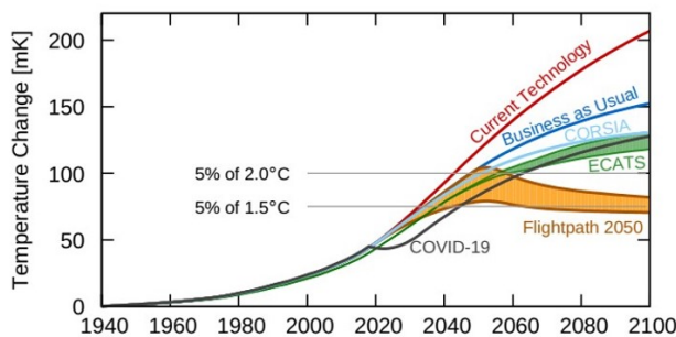
Figure 9.2: The horizontal lines indicate 5 % of a 2 °C and 1.5 °C climate target. The scenarios describe a future use of current technology, i.e. without technology improvements (CurTec, red), a business-as-usual future technological improvement (BAU, blue), the offsetting scheme of the international civil aviation organisation (CORSIA, light blue), and 2 Flightpath 2050 scenarios which differ in the speed of technology improvements (FP2050 and FP2050-cont, brown and orange, respectively).
