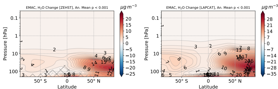
Figure A.15: Annual mean (2010-2014) of \text{H}_2\text{O} perturbation ( \mu\text{gm}^{-3} ) for the ZEHST scenario (left) and the LAPCAT scenario (right) for both models LMDZ-INCA (top) and EMAC (bottom). Hatched areas are characterized by a p-value higher than the threshold indicated in the title of each plot.
