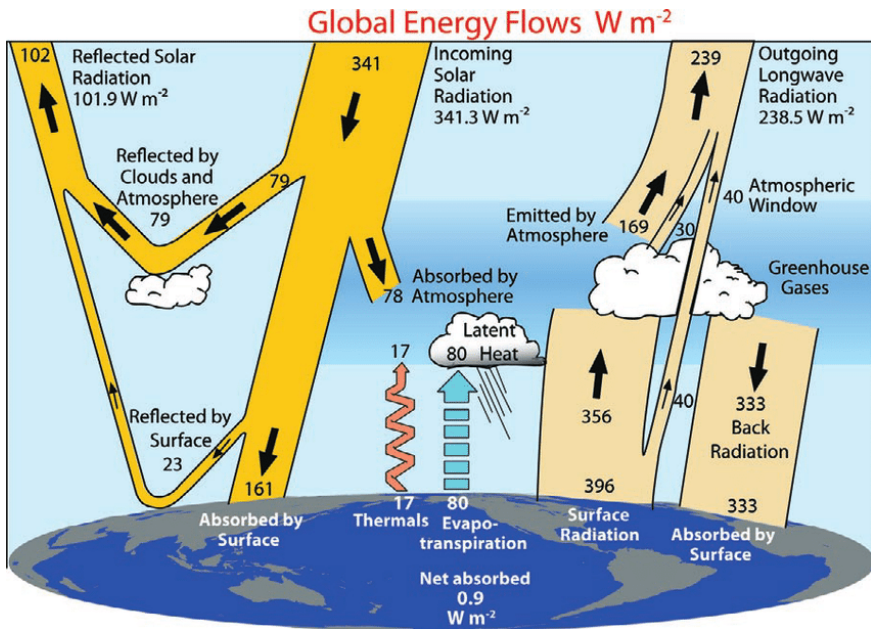
Figure 2.4: The global annual mean Earth's energy budget for the March 2000 to May 2004 period ( \text{W m}^{-2} ). The broad arrows indicate the schematic flow of energy in proportion to their importance. The figure and caption were published by Trenberth, Fasullo, and Kiehl [41]. The image was reproduced with permission of the rights holder, the American Meteorological Society .
