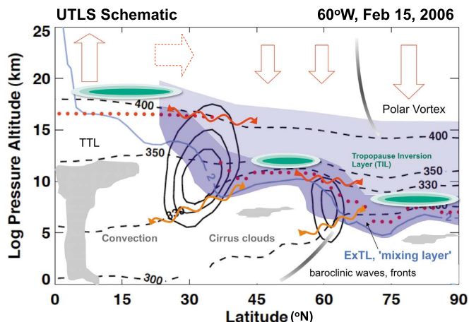
Figure 2.8: Schematic snapshot of the extratropical UTLS using data from a Northern Hemisphere section along 60° W longitude on 15 February 2006. Wind contours (solid black lines 10 ms -1 interval), potential temperature surfaces (dashed black lines), thermal tropopause (red dots), and potential vorticity surface (2 PVU: light blue solid line). Illustrated schematically are the Ex-UTLS (dark and light blue shading), ExTL (dark blue shading), clouds and fronts (gray shading), static stability contours in the TIL (green shading), quasi-isentropic exchange (red wavy arrows), cross-isentropic exchange (orange wavy arrows), and the Brewer-Dobson circulation (deep, red solid outline; shallow, dotted solid outline). The figure and caption were published by Gettelman et al. [73] and is free for non-commercial use according to Wiley's terms and conditions.
