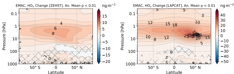
Figure A.13: Annual mean (2010-2014) of \text{HO}_x perturbation ( \text{ngm}^{-3} ) for the ZEHST scenario (left) and the LAPCAT scenario (right) for EMAC. hatched areas are characterized by a p-value higher than the threshold indicated in the title of each plot.
