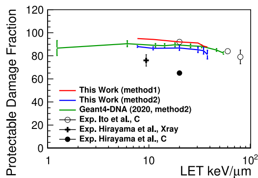
Fig. 5. Protectable damage fraction (fraction of indirect damage) as a function of LET. Method1 is result of the calculation based on SF. Method2 is result of the calculation based on the damage classification. The experimental data on the V79 cell line are estimated as protectable damage fraction at the infinite DMSO concentration [54,55].
