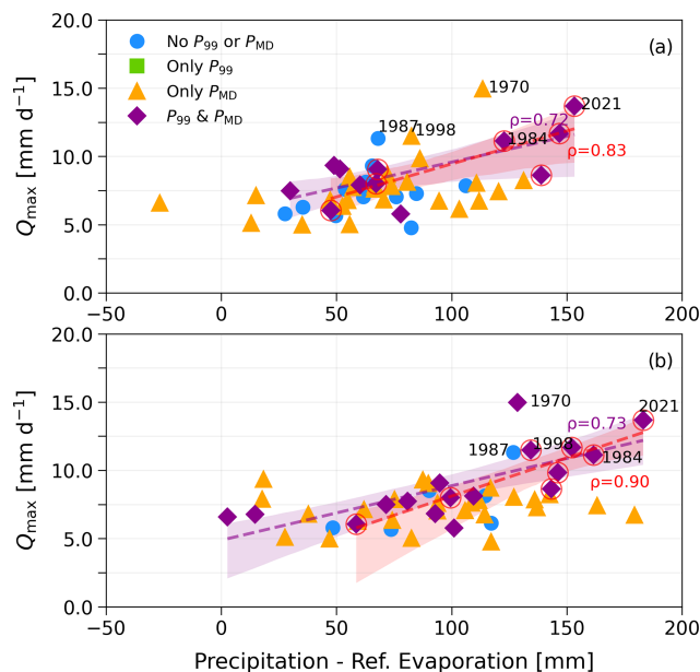
Figure 7. Annual maxima events ( Q_{\max} ) and their 30 d pre-event effective rainfall at Maastricht (a) and Vaals (b), including their preceding extreme indicators. The top five floods during the study period are shown with their year of occurrence. The dashed purple line represents the linear fit, using the least-squares approach, between the effective rainfall of the high-flow events preceded by P_{99} and P_{MD} and their respective Q_{\max} values, while the red dashed line represents the linear fit between the effective rainfall of the Compound-III events and their Q_{\max} . The shaded areas show the 95 % confidence intervals for the fits, and the Pearson correlation coefficients ( \rho ) are also reported.
