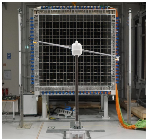
Figure 4. Model wind turbine in front of 3 m x 3 m active grid.
