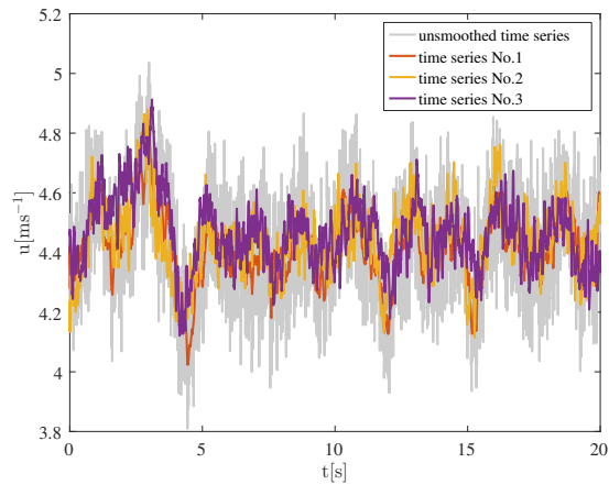
Figure 6. Wind speed time series behind the active grid using the gust excitation protocol
