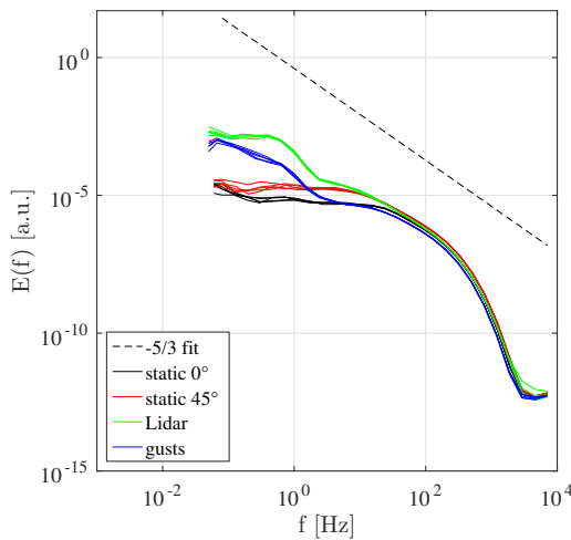
Figure 7. Power spectra of the four different test cases.
