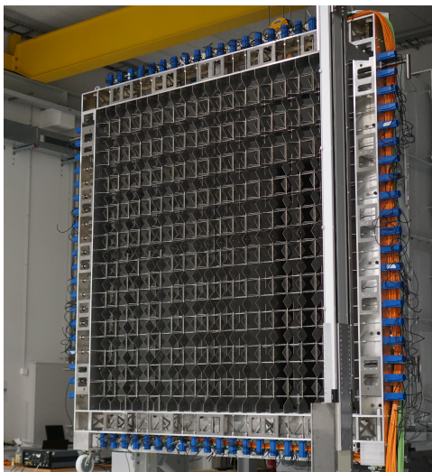
Figure 2. Active grid mounted to the wind tunnel nozzle.
