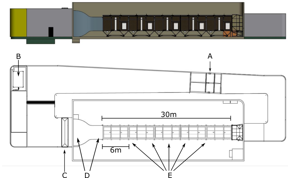
Figure 1. Schematic of the WindLab wind tunnel of the University of Oldenburg (above: side view; below: top view).
