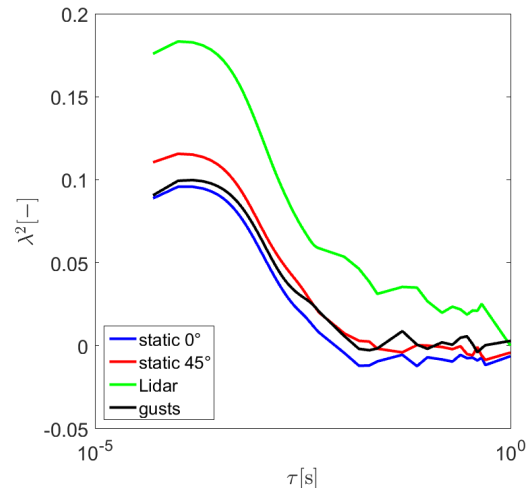
Figure 8. Shape parameter \lambda^2 of the four different test cases.
