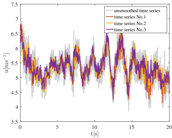
Figure 5. Wind speed time series behind the active grid using the LiDAR excitation protocol
