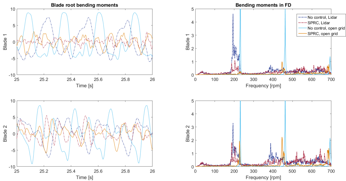
Figure 9. Blade loads and blade root loads in the frequency domain (FD) for no control and SPRC for laminar and turbulent inflow
