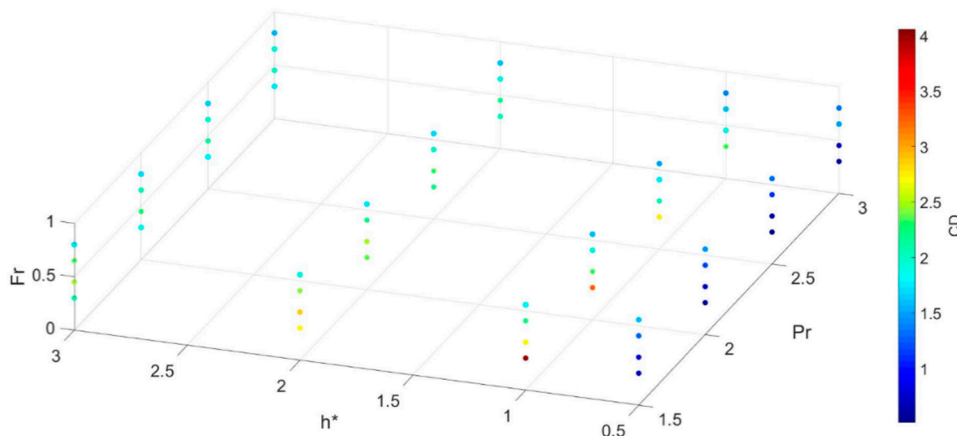
Figure 25. Drag coefficient for box deck based on the proximity ratio ( Pr=1.5, 2, 2.5, 3 ), inundation ratio ( h^*=0.5, 1, 2, 3 ), and Froude number ( Fr=0.30, 0.45, 0.65, 0.80 ). These drag coefficients hold for a rectangular deck with an aspect ratio (height:width) of 0.27.
