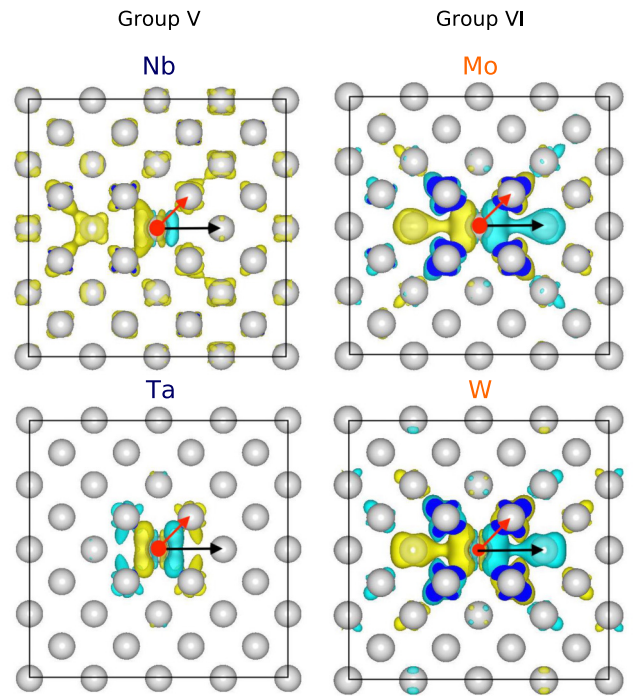
FIG. 6. Change in ILDOS when an atom is displaced by 0.015 Å towards the 2NN relative to the ideal structure projected along the (001) plane. The isosurface value of the ILDOS has been optimized for best visualization. Yellow and blue are negative and positive values of the change in ILDOS, respectively.
