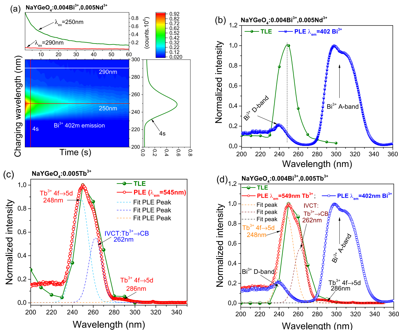
Fig. 9. (a) 2D contour plot of RT iso-thermal decay curves as a function of charging wavelength for NaYGeO 4 :0.004Bi 3+ , 0.005Nd 3+ . A comparison of TL excitation (TLE) curves with the PL excitation (PLE) spectra for (b) NaYGeO 4 :0.004Bi 3+ , 0.005Nd 3+ , (c) NaYGeO 4 :0.005Tb 3+ , and (d) NaYGeO 4 :0.004Bi 3+ , 0.005Tb 3+ . The PLE spectra of NaYGeO 4 :0.005Tb 3+ (λ em = 545 nm) and NaYGeO 4 :0.004Bi 3+ (λ em = 402 nm) recorded at RT are also given in (c)-(d).
