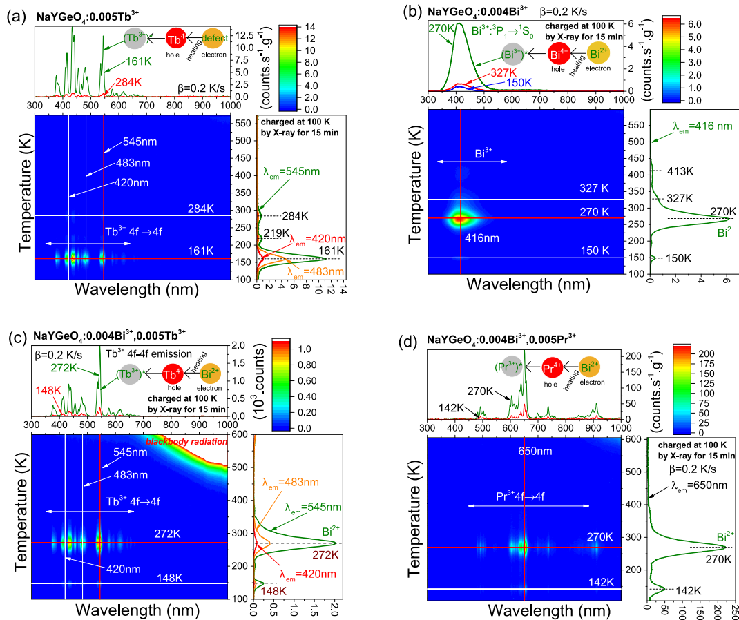
Fig. 4. Low-temperature thermoluminescence (TL) emission spectra for (a) NaYGeO 4 :0.005Tb 3+ , (b) NaYGeO 4 :0.004Bi 3+ , (c) NaYGeO 4 :0.004Bi 3+ , 0.005Tb 3+ , and (d) NaYGeO 4 :0.004Bi 3+ , 0.005Pr 3+ after exposure to X-ray charging at 100 K. The used heating rate is 0.2 K/s in (a)–(d).
