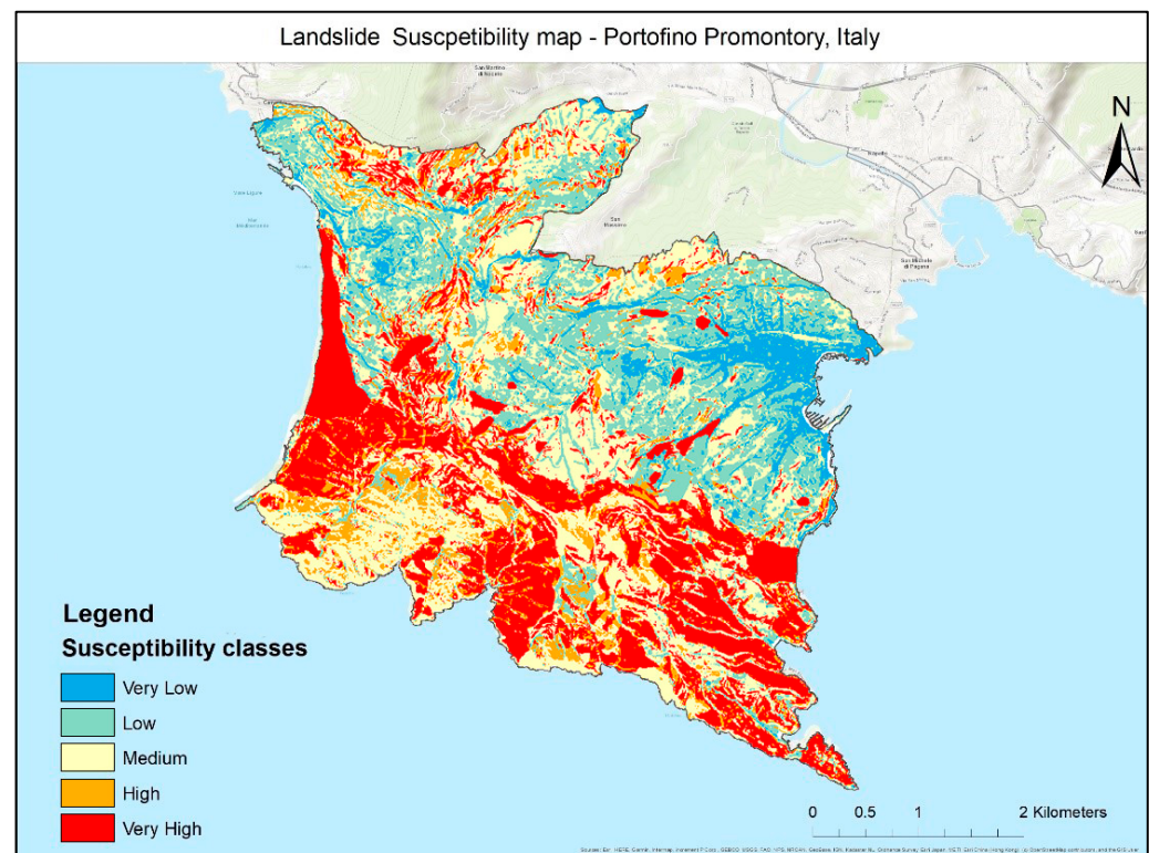
Figure 3. Landslide susceptibility map.
