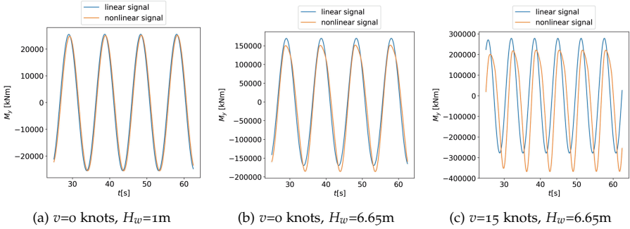
Figure 4.7: Loading cases
