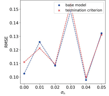
(d) Graph depicting the relationship between RMSE and \sigma_n
