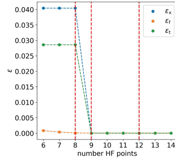
(b) Tracking \epsilon throughout the optimization process
