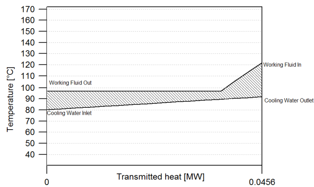
(a) Condenser (This Work)
