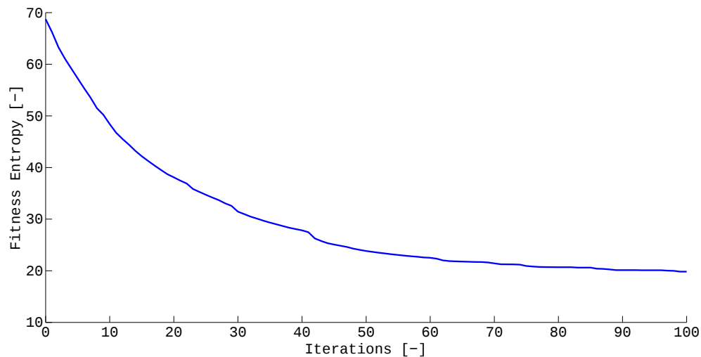
Figure 4-2: Fitness entropy during each iteration in Latin Hypercube Sampling
