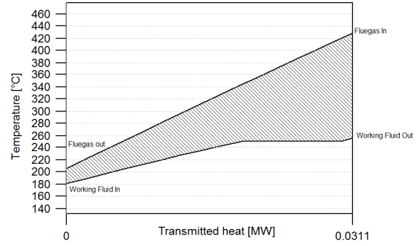
(b) EGR Evaporator (This Work)
