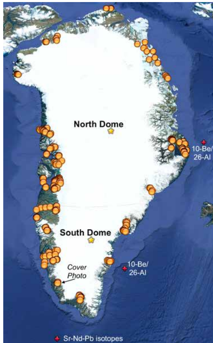
Figure 1: Location of ^{10}\text{Be} ages (yellow circles), basal ice and bedrock samples (stars), and marine sediment cores (red crosses) constraining Greenland ice-sheet paleo history. Location of issue cover photo from Nigerdlikasik Bræ denoted by arrow.
