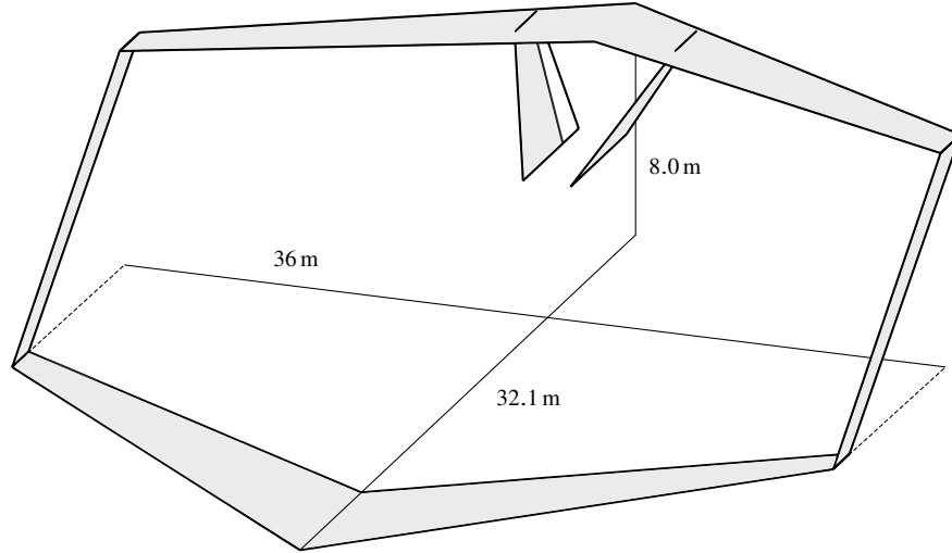
Fig. 5 Staggered box-wing geometry under investigation.
