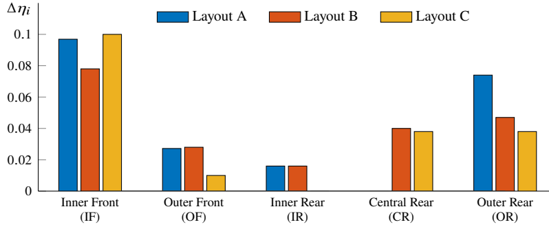
Fig. 14 CS span comparison among Layouts A, B and C.
