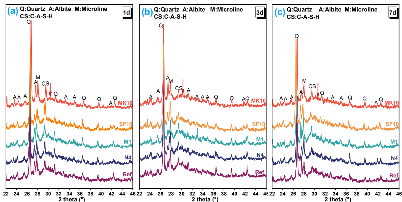
Figure 7. XRD patterns of AASF pastes cured for (a) 1 day, (b) 3 days, and (c) 7 days. (Quartz: \text{SiO}_2 , albite: \text{NaAlSi}_3\text{O}_8 , and microcline: \text{KAlSi}_3\text{O}_8 ).
