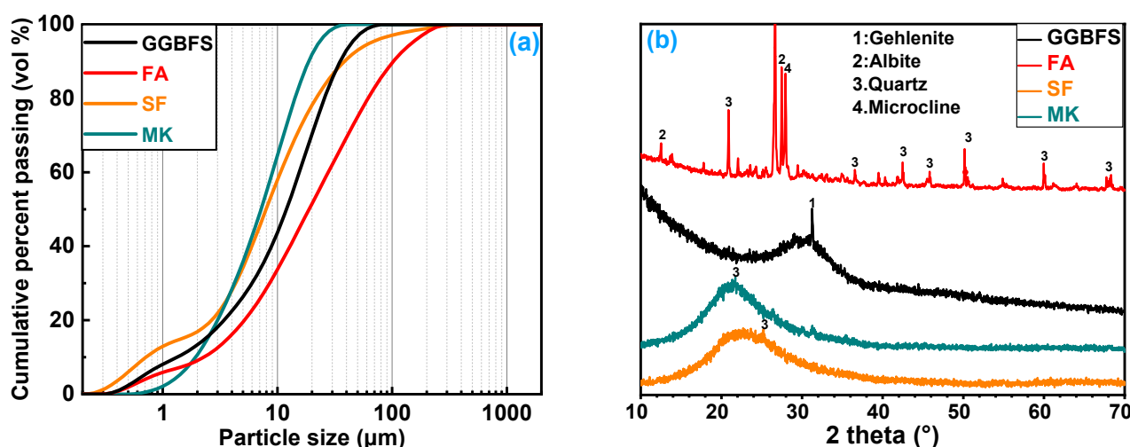
Figure 1. Particle size distribution (a,b) XRD pattern of raw materials (ground granulated blast-furnace slag (GGBFS), fly ash (FA), Silica fume (SF) and metakaolin (MK)). (Gehlenite: \text{Ca}_2\text{Al}_2\text{SiO}_7 , albite: \text{NaAlSi}_3\text{O}_8 , quartz: \text{SiO}_2 , and microcline: \text{KAlSi}_3\text{O}_8 ).
